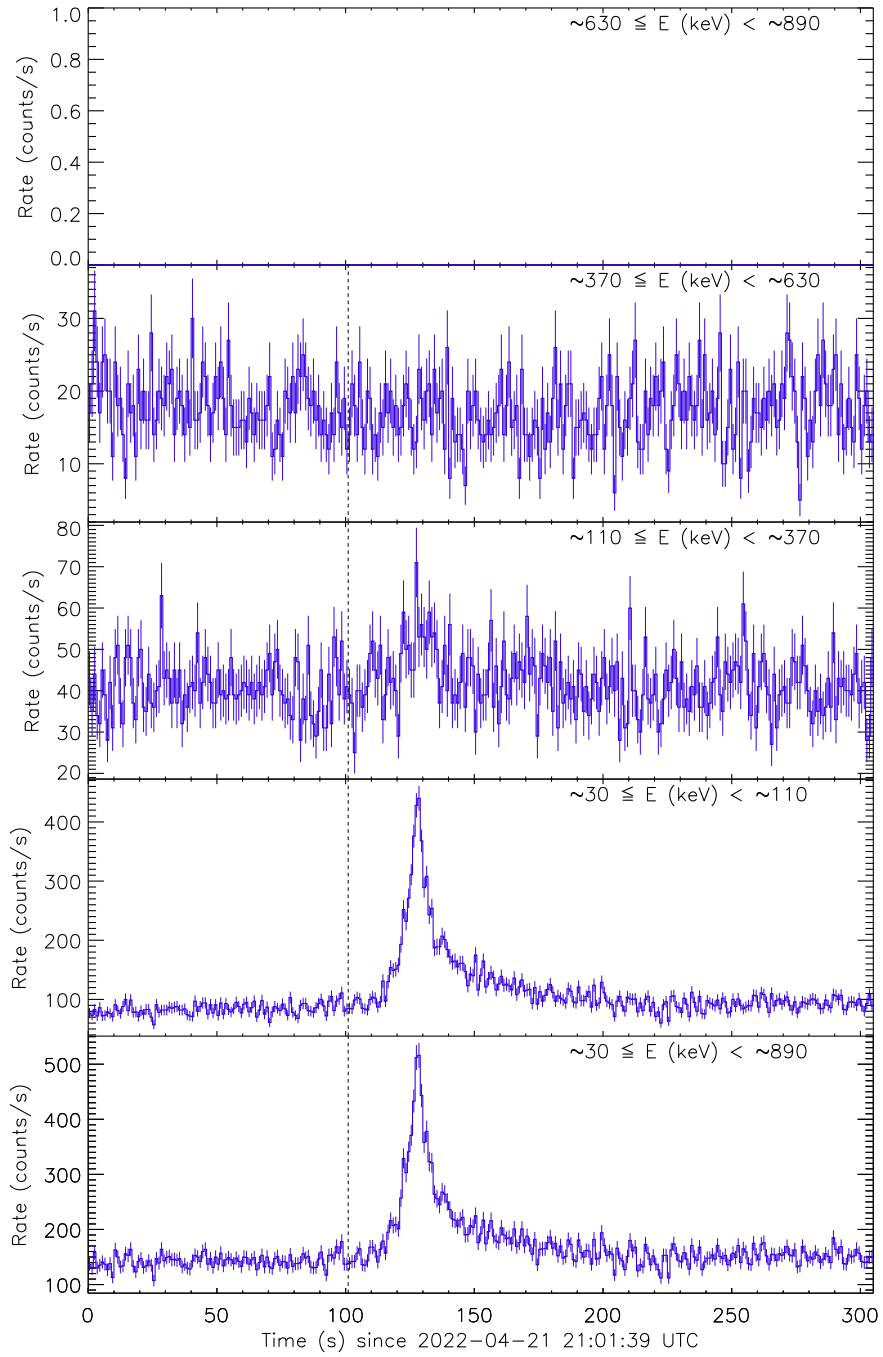
Figure 4: Raw count rate curve of a burst recorded by the detector unit no. 1. The vertical dashed line marks the trigger time by GECAM.
