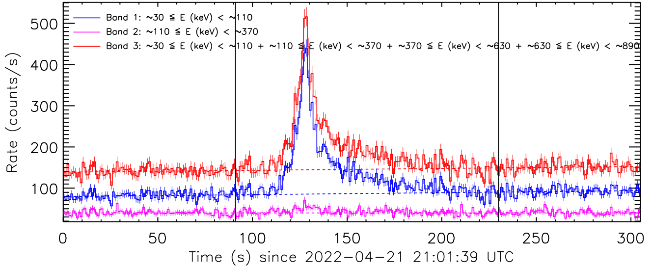
Figure 5: Background fit to the data from the detector unit no. 1 by a linear function. Pre-burst and post-burst intervals were used for the background fit which are delimited by the vertical solid lines.
