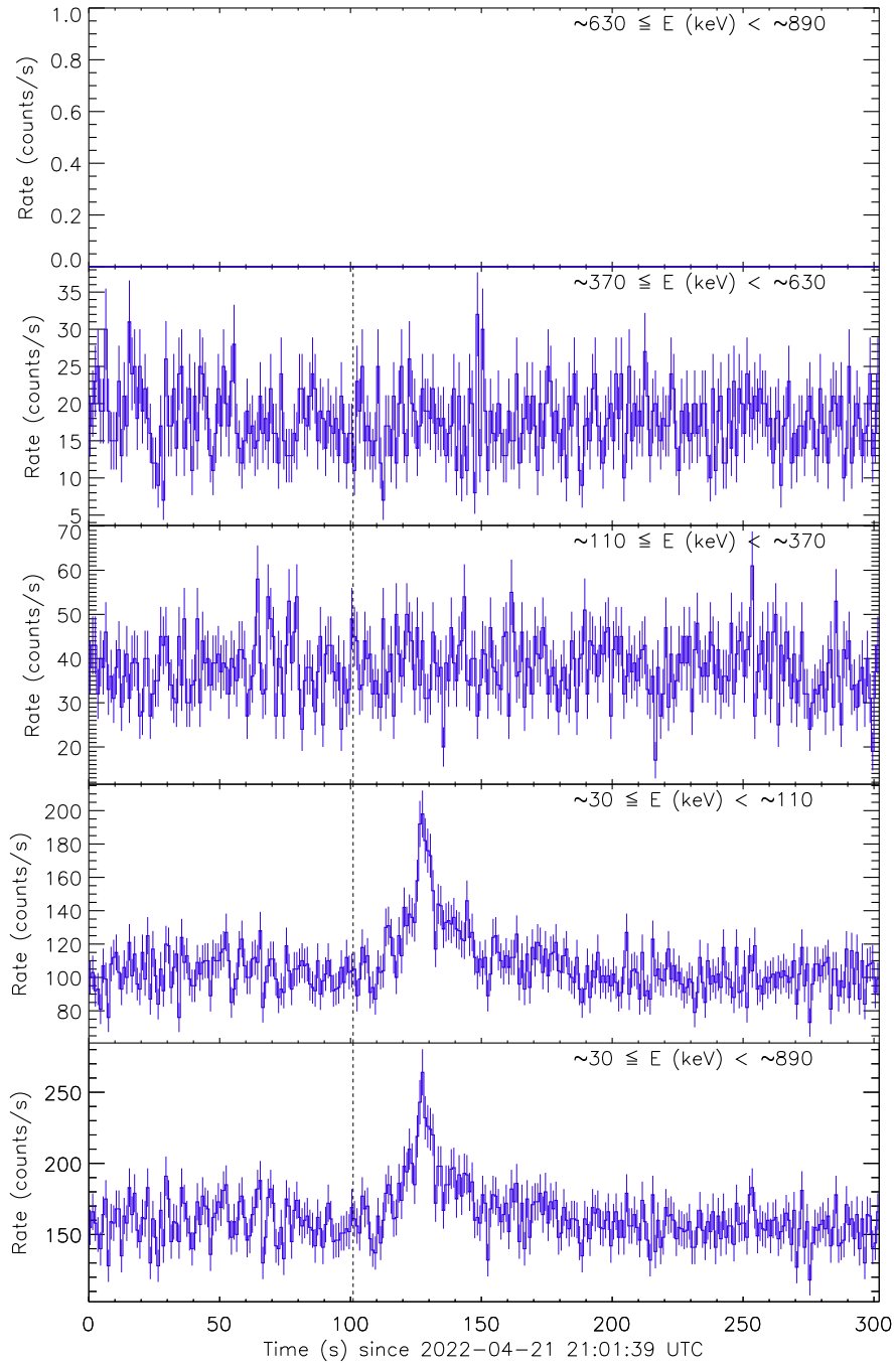
Figure 1: Raw count rate curve of a burst recorded by the detector unit no. 0. The vertical dashed line marks the trigger time by GECAM.
