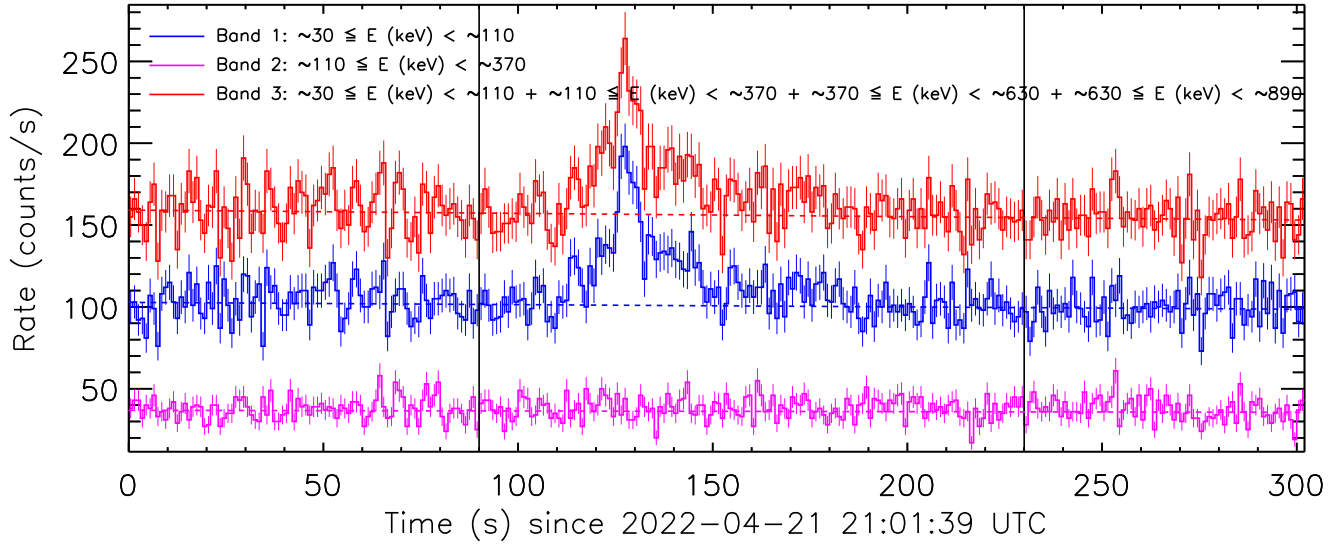
Figure 2: Background fit to the data from the detector unit no. 0 by a linear function. Pre-burst and post-burst intervals were used for the background fit which are delimited by the vertical solid lines.
