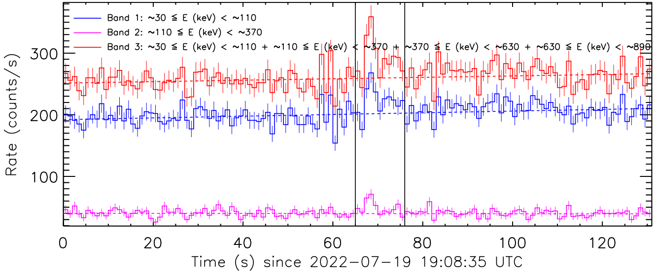
Figure 2: Background fit to the data from the detector unit no.1 by a linear function. The pre-burst and post-burst intervals used for the background fit are delimited by the vertical solid lines.
