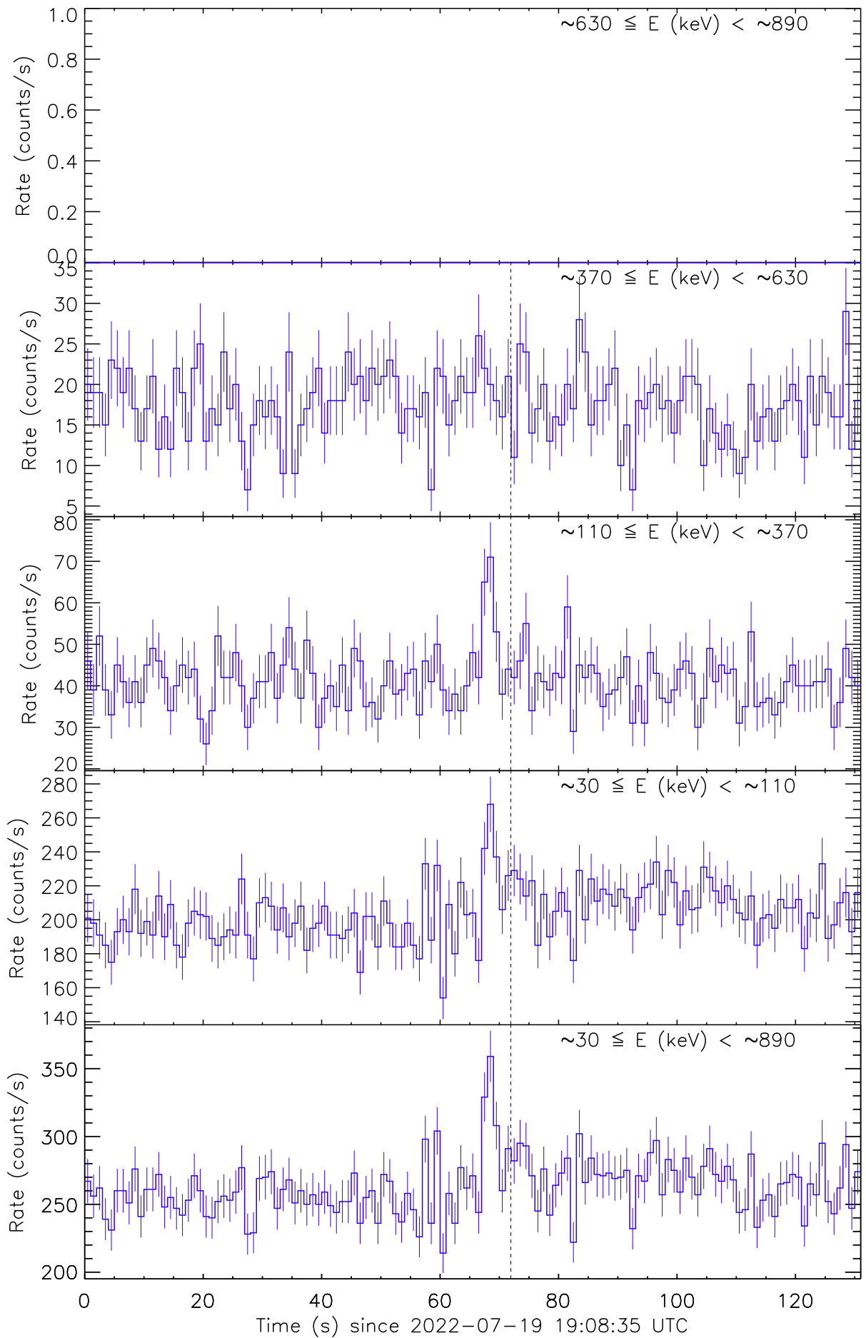
Figure 1: Raw count rate curve of GRB 220719A recorded by the detector unit no. 1. The vertical dashed line marks the trigger time by KONUS-Wind.
