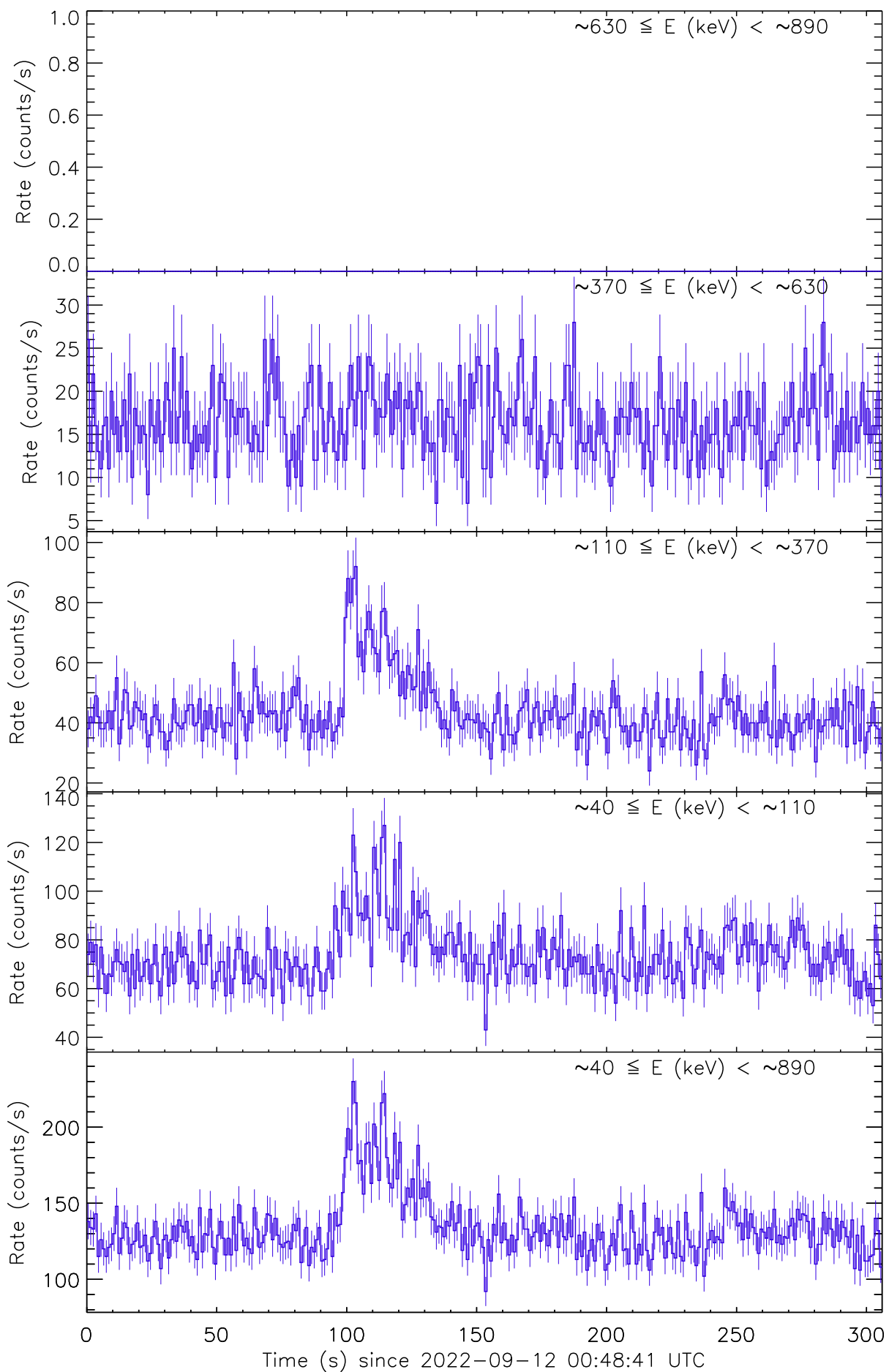
Figure 1: Raw count rate curve of GRB 220912A recorded by the detector unit no. 1.
