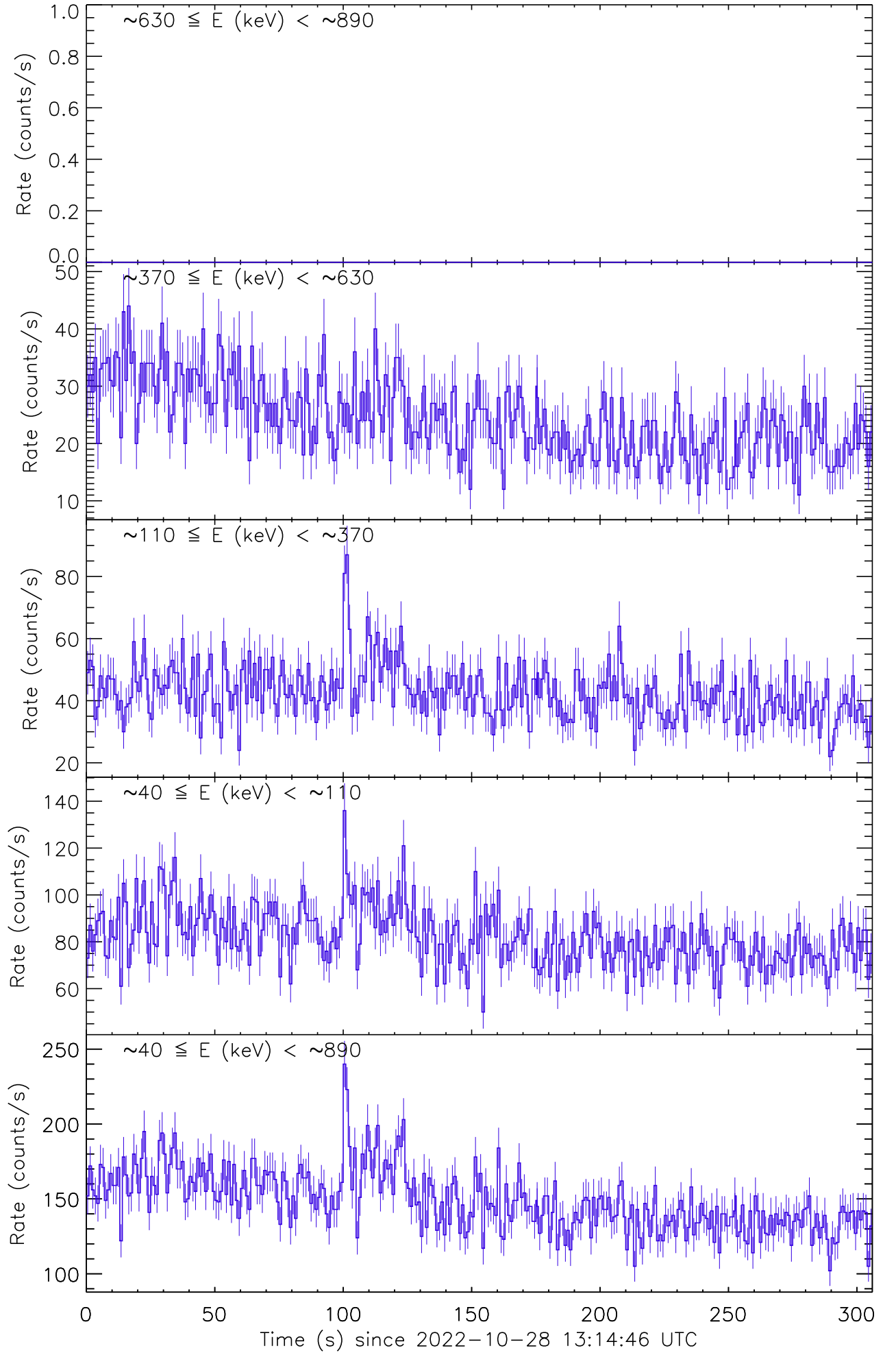
Figure 1: Raw count rate curves of GRB 221028A recorded by the detector unit no. 0.
