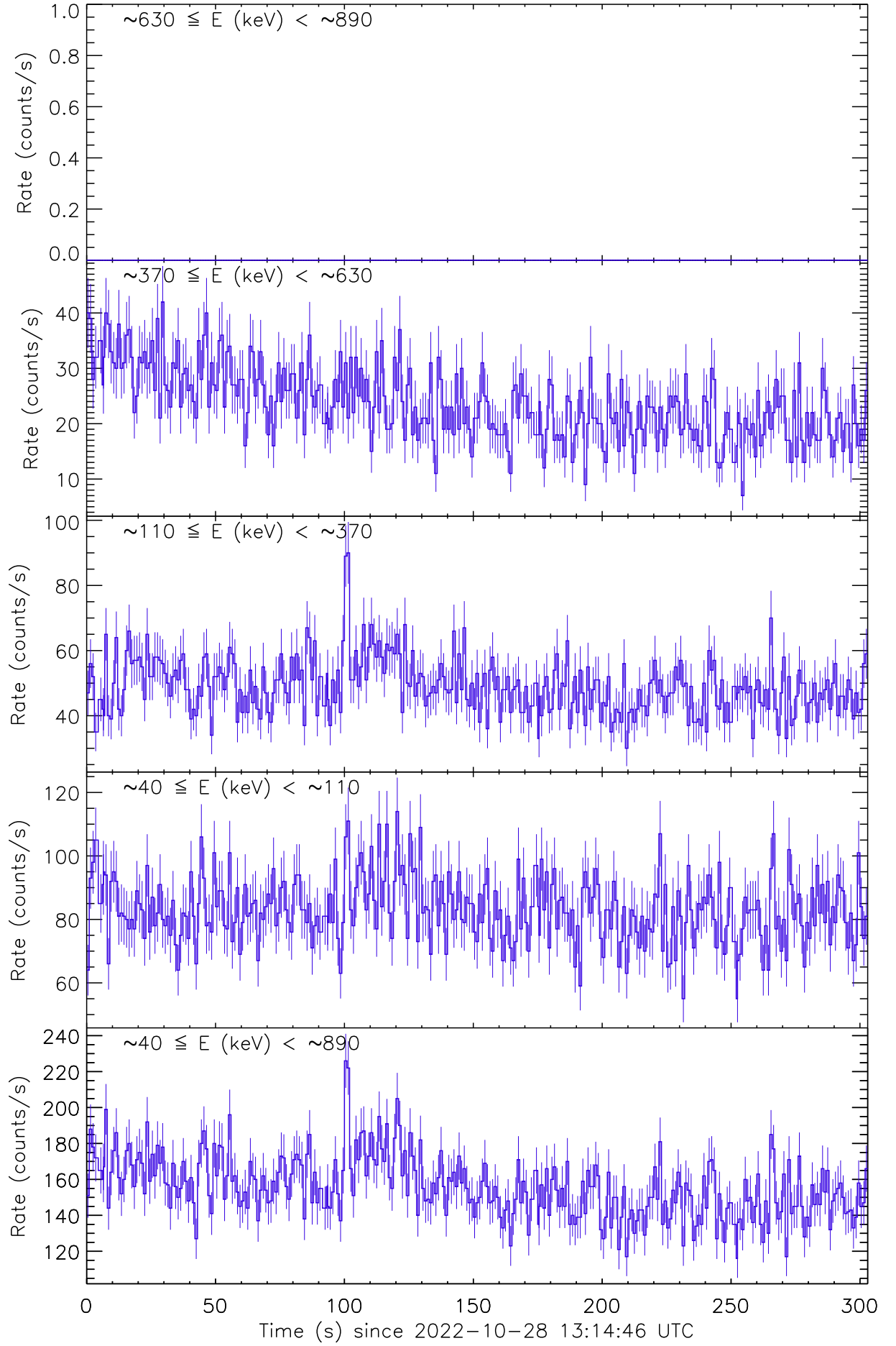
Figure 4: Raw count rate curves of GRB 221028A recorded by the detector unit no. 1.
