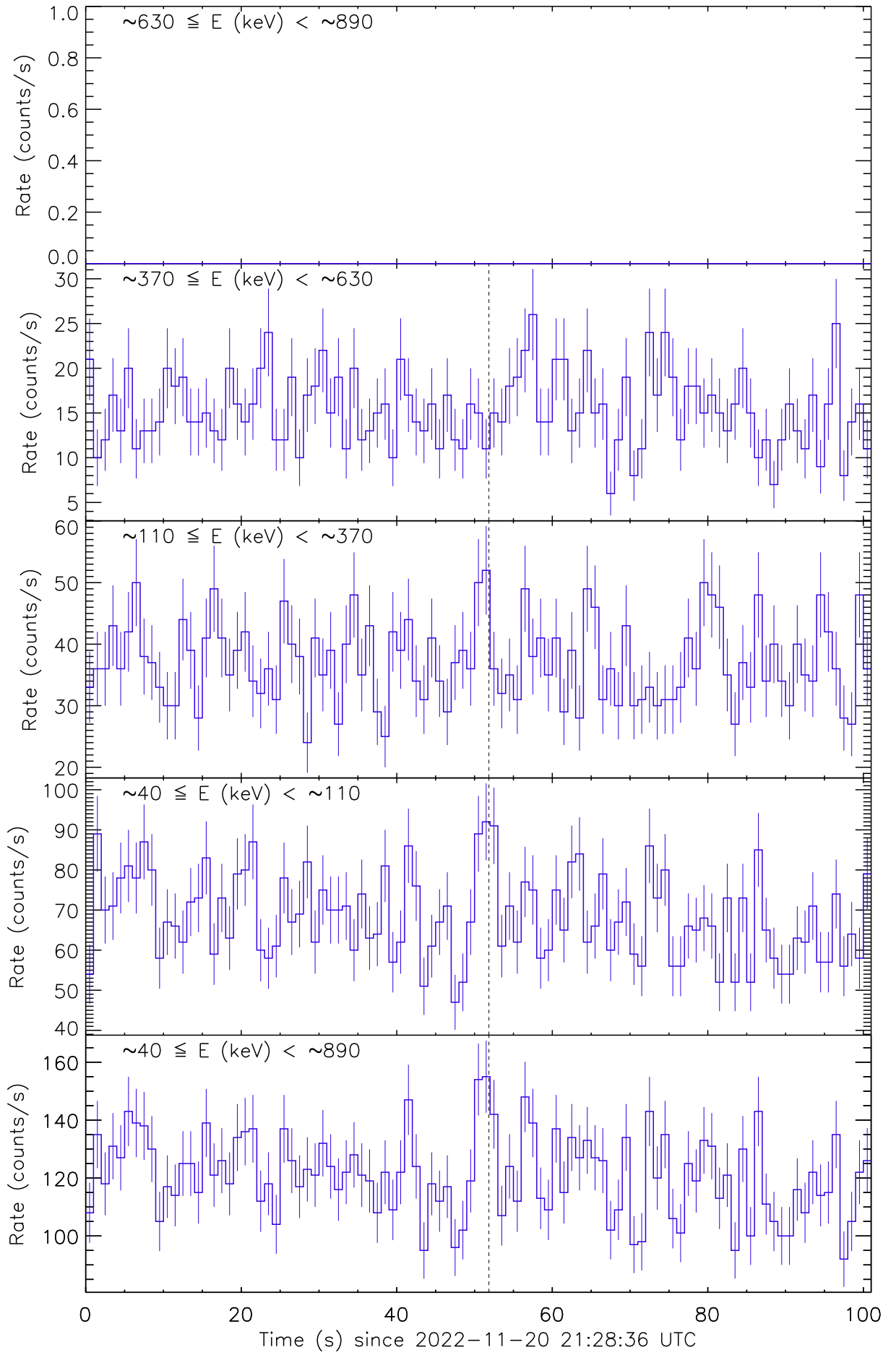
Figure 1: Raw count rate curves of GRB 221120A recorded by the detector unit no. 1. The vertical dashed line marks the trigger time by FERMI/GBM.
