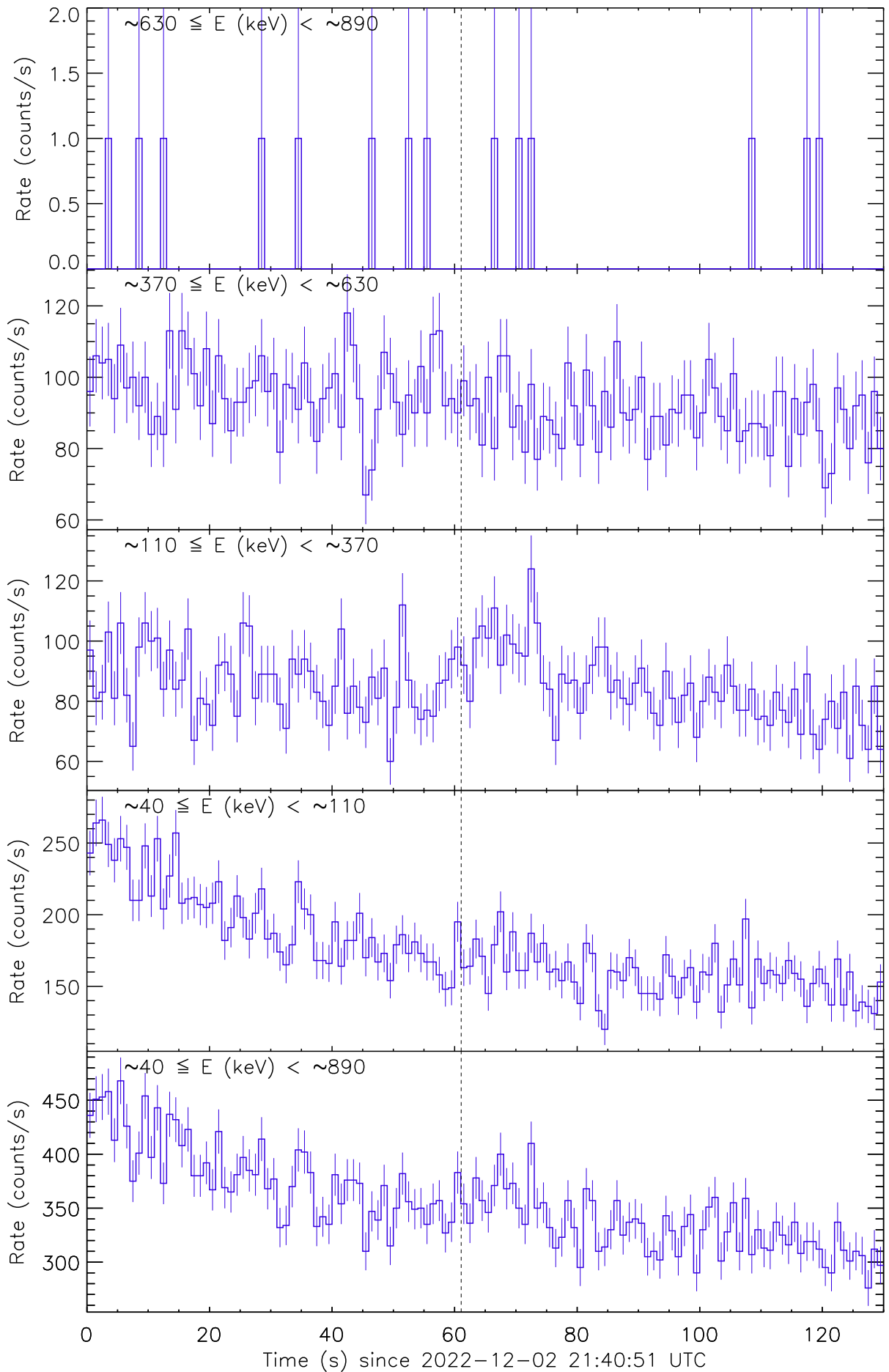
Figure 1: Raw count rate curves of GRB 221202B recorded by the detector unit no. 1. The vertical dashed line marks the trigger time by Fermi/GBM.
