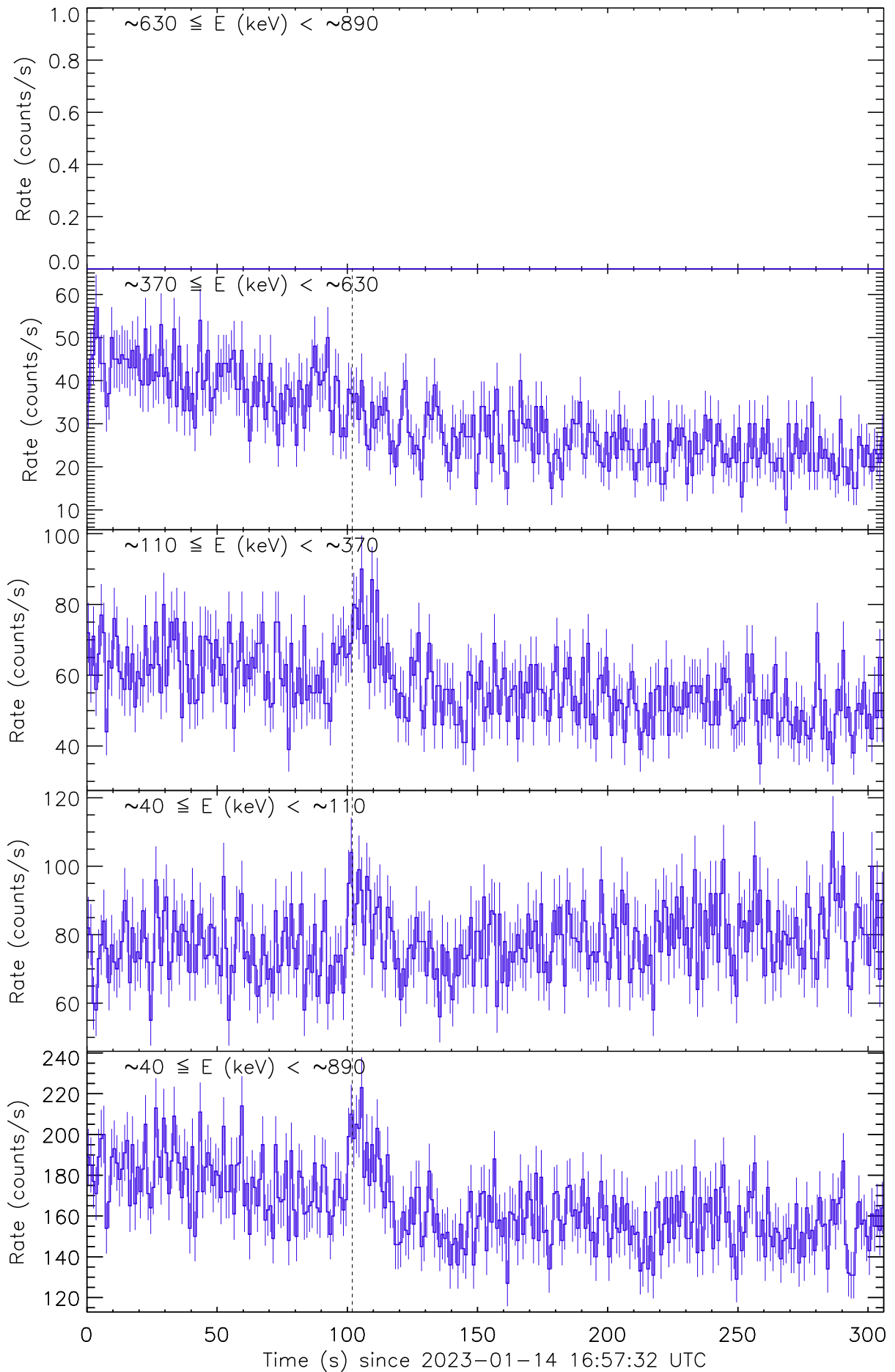
Figure 1: Raw count rate curves of GRB 230114A recorded by the detector unit no. 1. The vertical dashed line marks the trigger time by Fermi/GBM.
