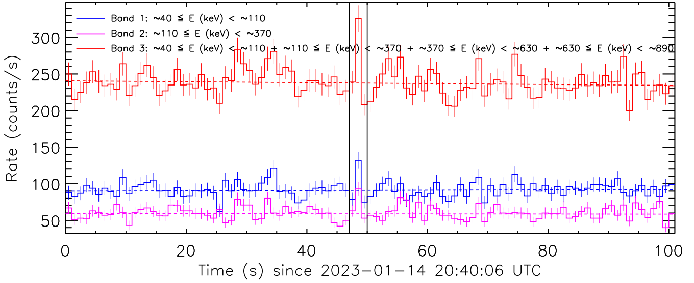
Figure 2: Background fit to the data from the detector unit no.1 by a linear function. The pre-burst and post-burst intervals which were used for the background fit are delimited by the vertical solid lines.
