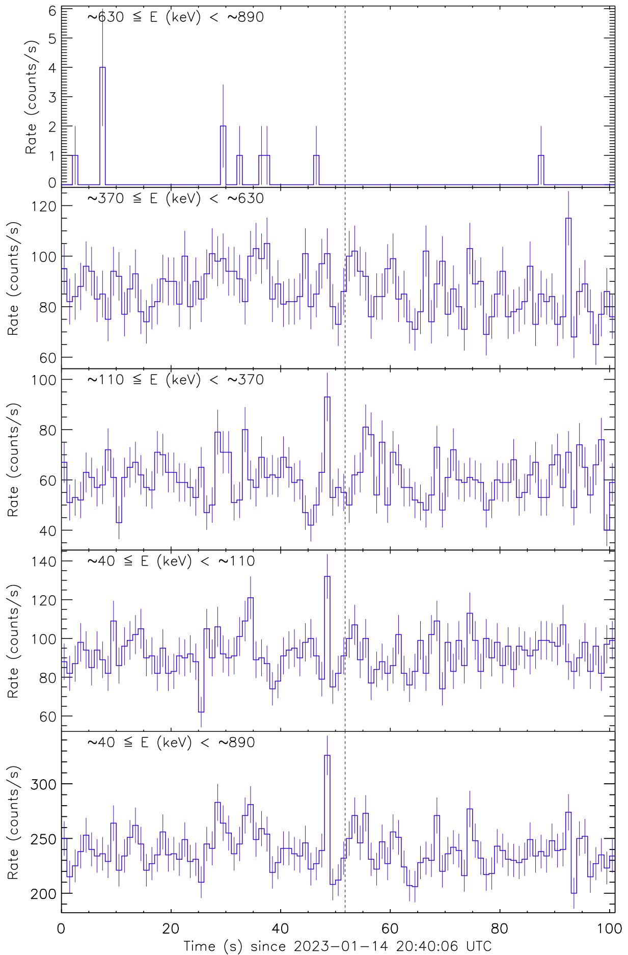
Figure 1: Raw count rate curves of GRB 230114B recorded by the detector unit no. 1. The vertical dashed line marks the trigger time by Konus-Wind.
