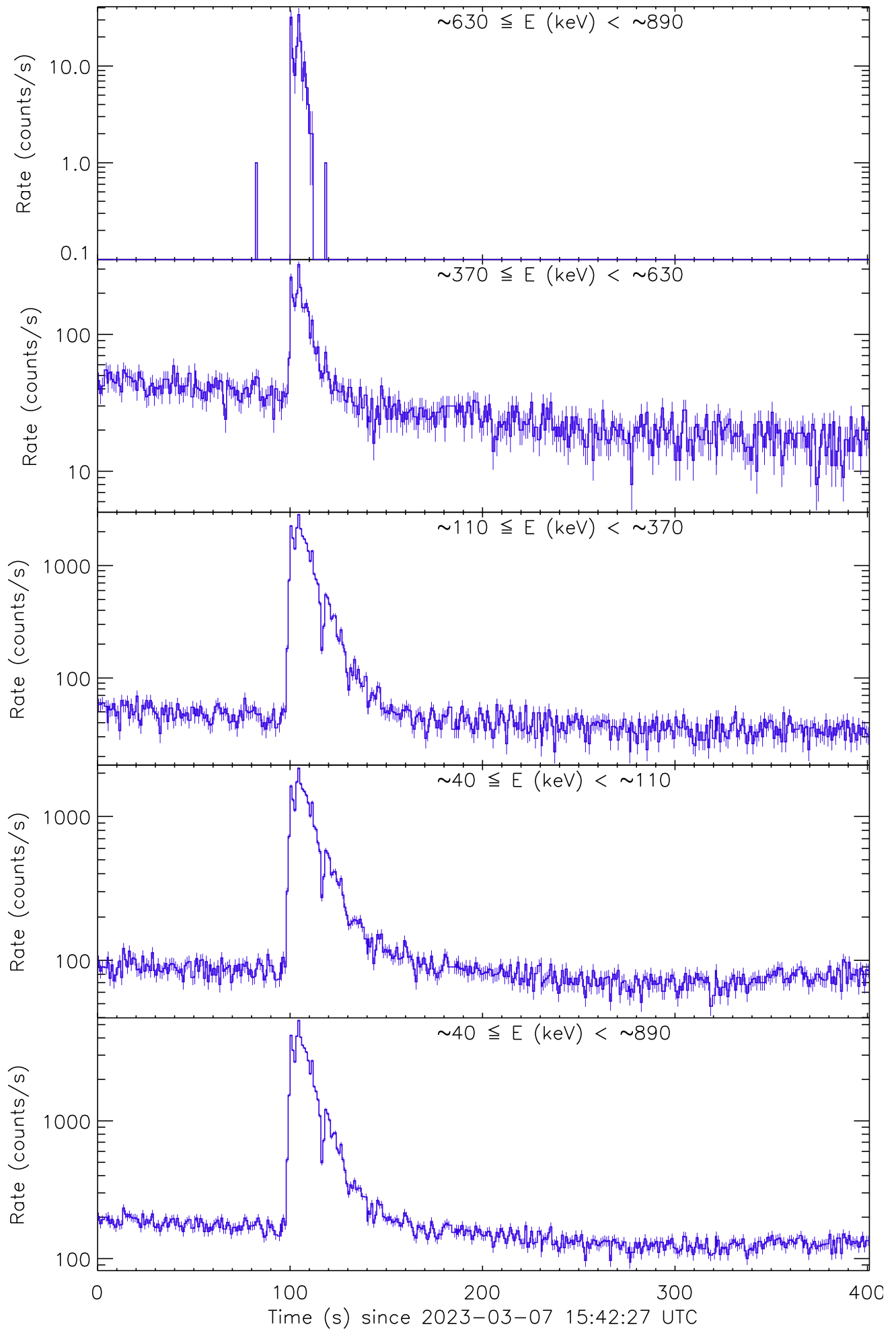
Figure 1: Raw count rate curves of GRB 230307A recorded by the detector unit no. 0.
