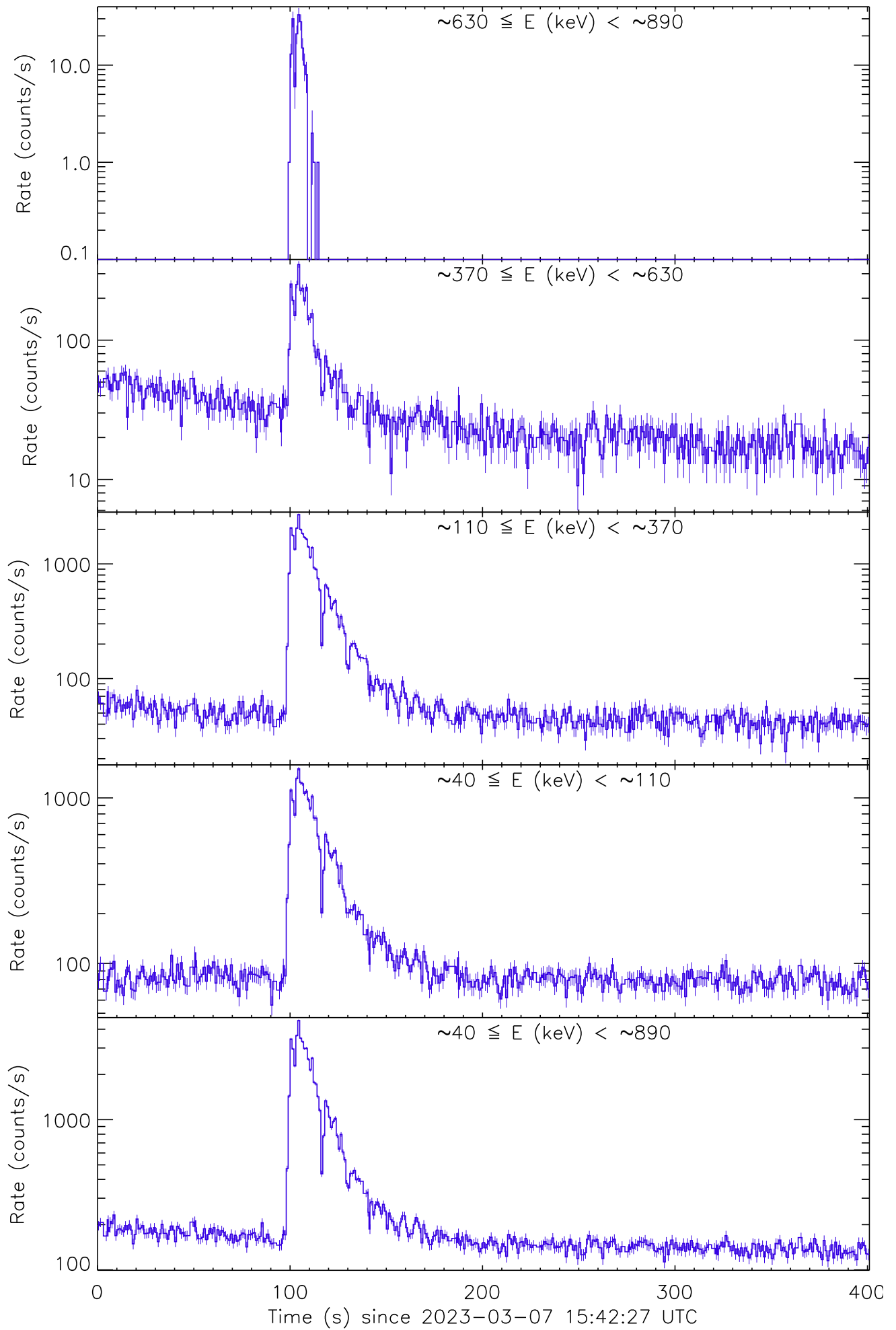
Figure 4: Raw count rate curves of GRB 230307A recorded by the detector unit no. 1.
