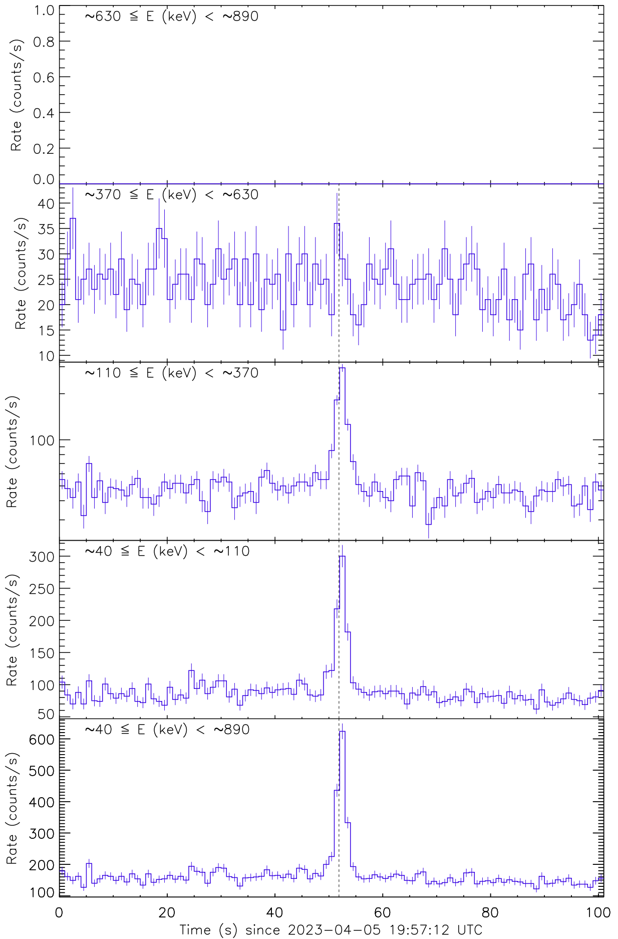
Figure 1: Raw count rate curves of GRB 230405B recorded by the detector unit no. 1. The vertical dashed line marks the trigger time by Fermi/GBM.
