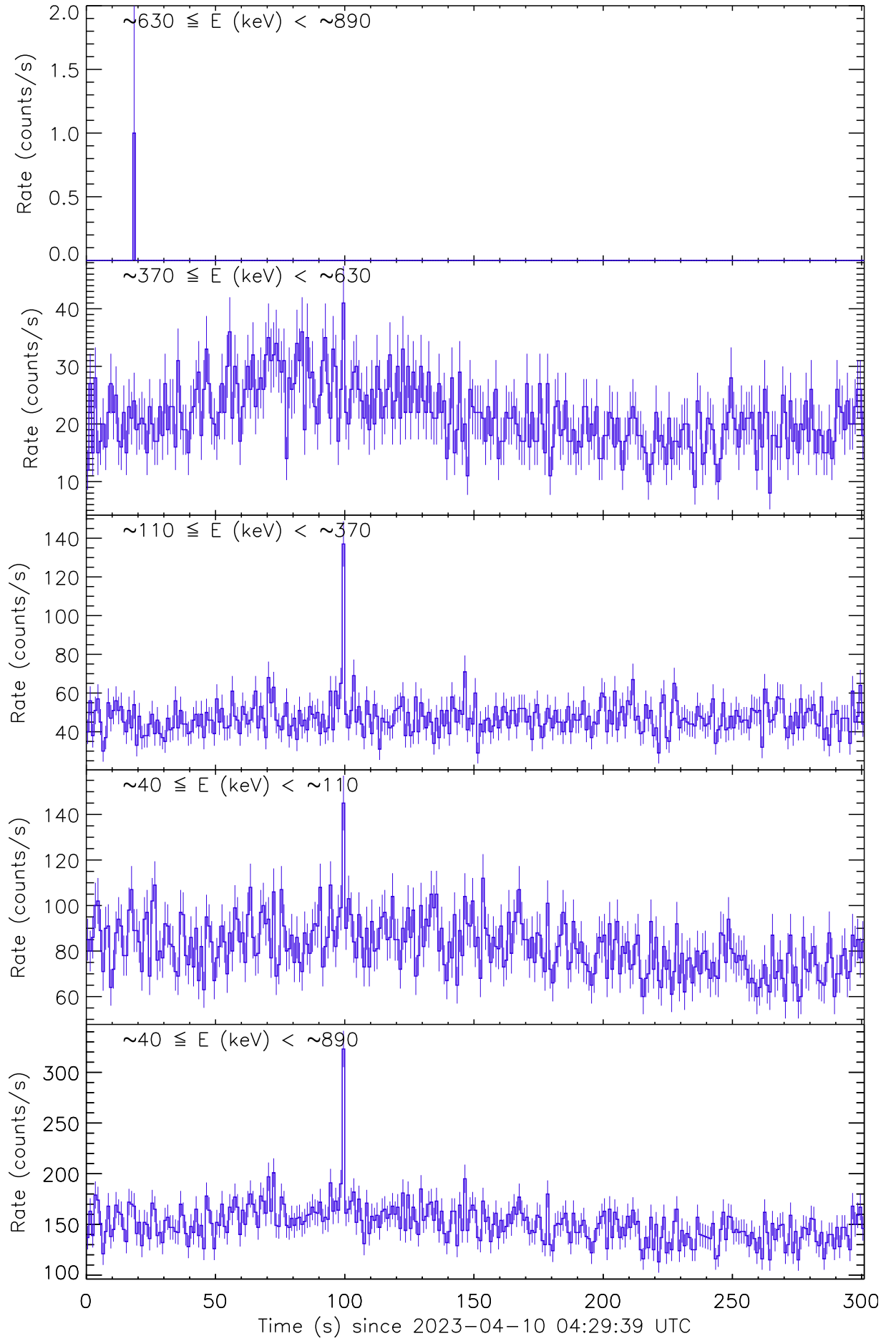
Figure 1: Raw count rate curves of GRB 230410B recorded by the detector unit no. 1.
