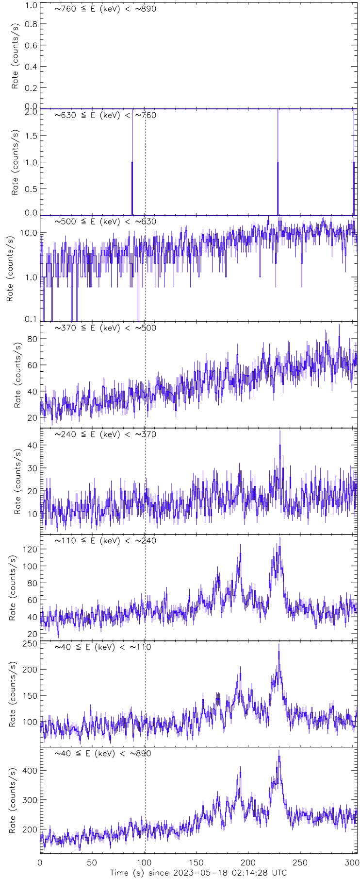
Figure 1: Raw count rate curves of GRB 230518B recorded by the detector unit no. 1. The vertical dashed line marks the trigger time by Fermi/GBM.
