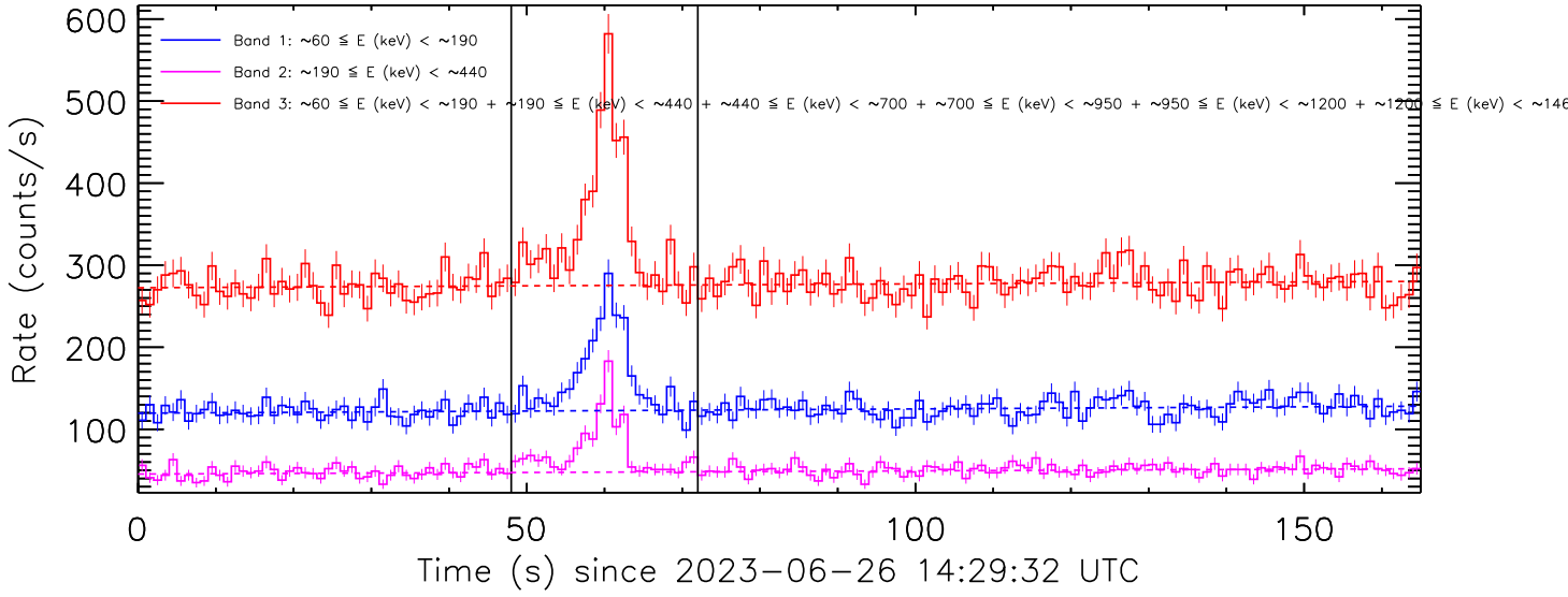
Figure 2: Background fit to the data from the detector unit no. 1 by a linear function. The pre-burst and post-burst intervals which were used for the background fit are delimited by the vertical solid lines.
