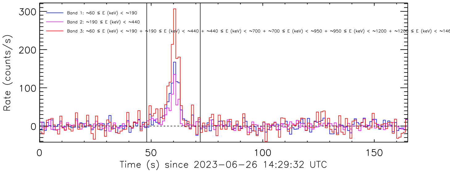
Figure 3: Background-subtracted count rate curves from the detector unit no. 1.
