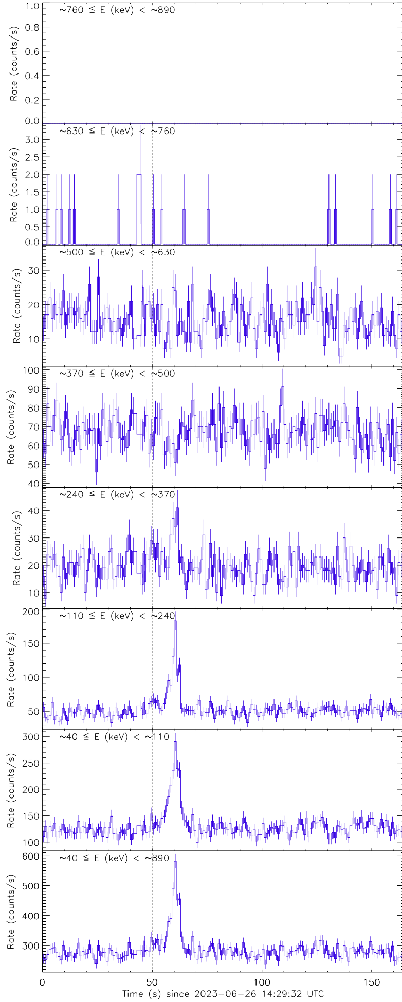
Figure 1: Raw count rate curves of GRB 230626A recorded by the detector unit no. 1. The vertical dashed line marks the trigger time by Fermi/GBM.
