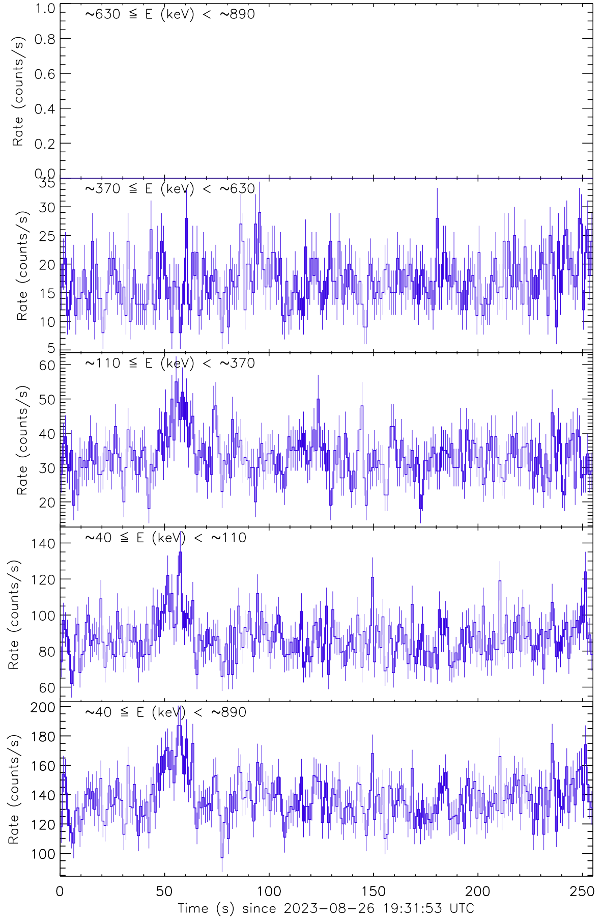
Figure 1: Raw count rate curves of GRB 230826A recorded by the detector unit no. 0.
