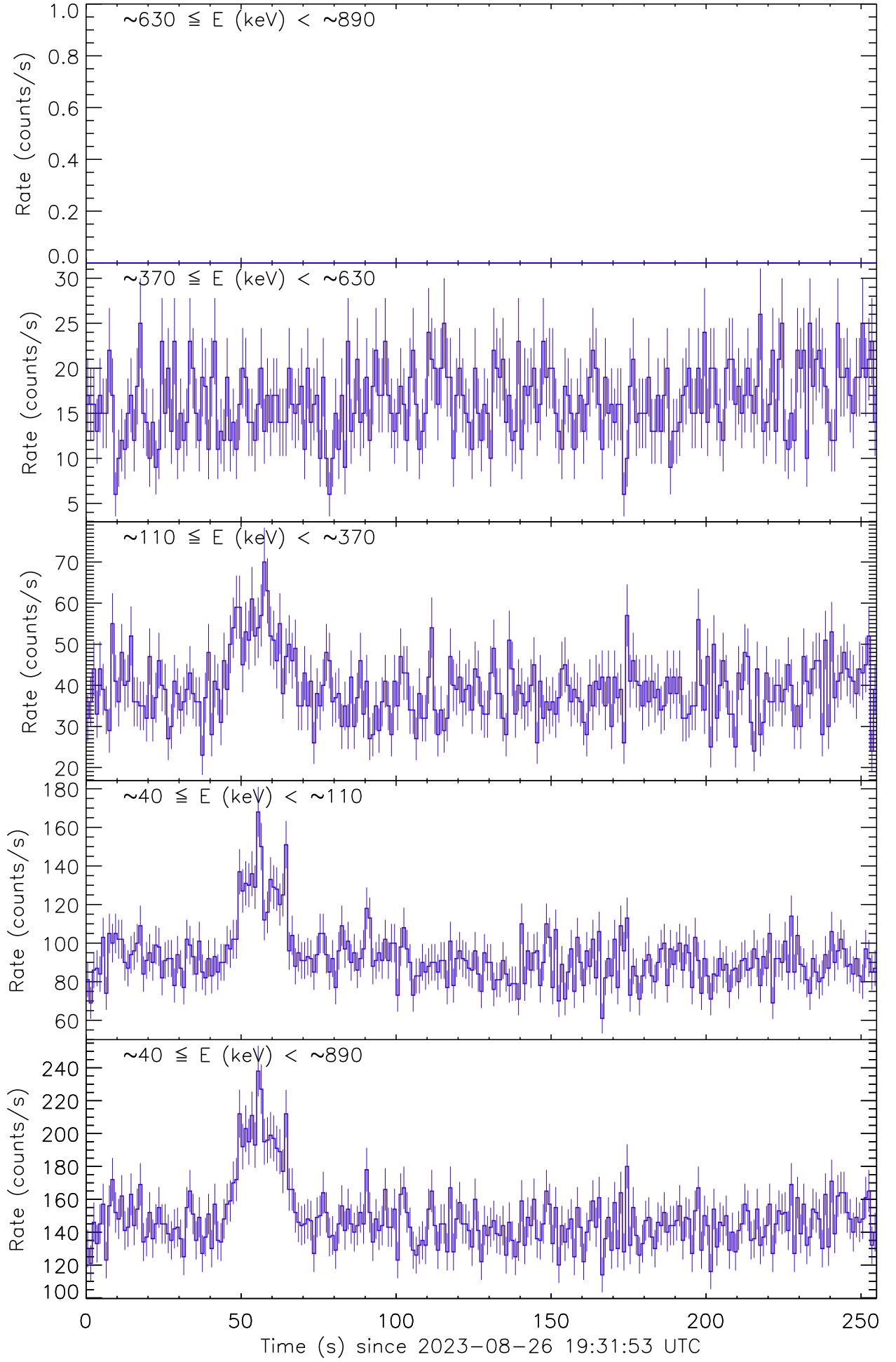
Figure 4: Raw count rate curves of GRB 230826A recorded by the detector unit no. 1.
