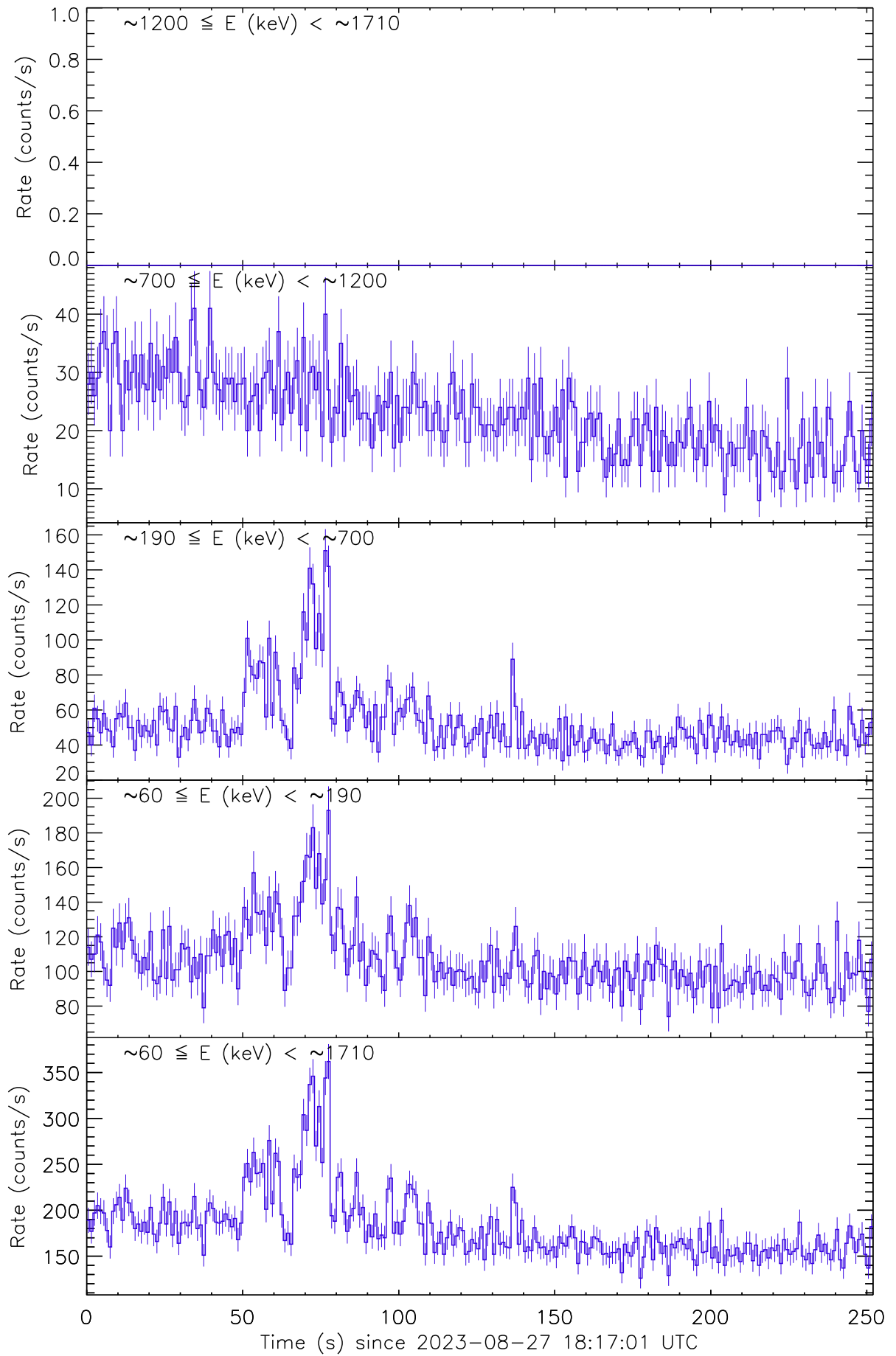
Figure 4: Raw count rate curves of GRB 230827A recorded by the detector unit no. 1.
