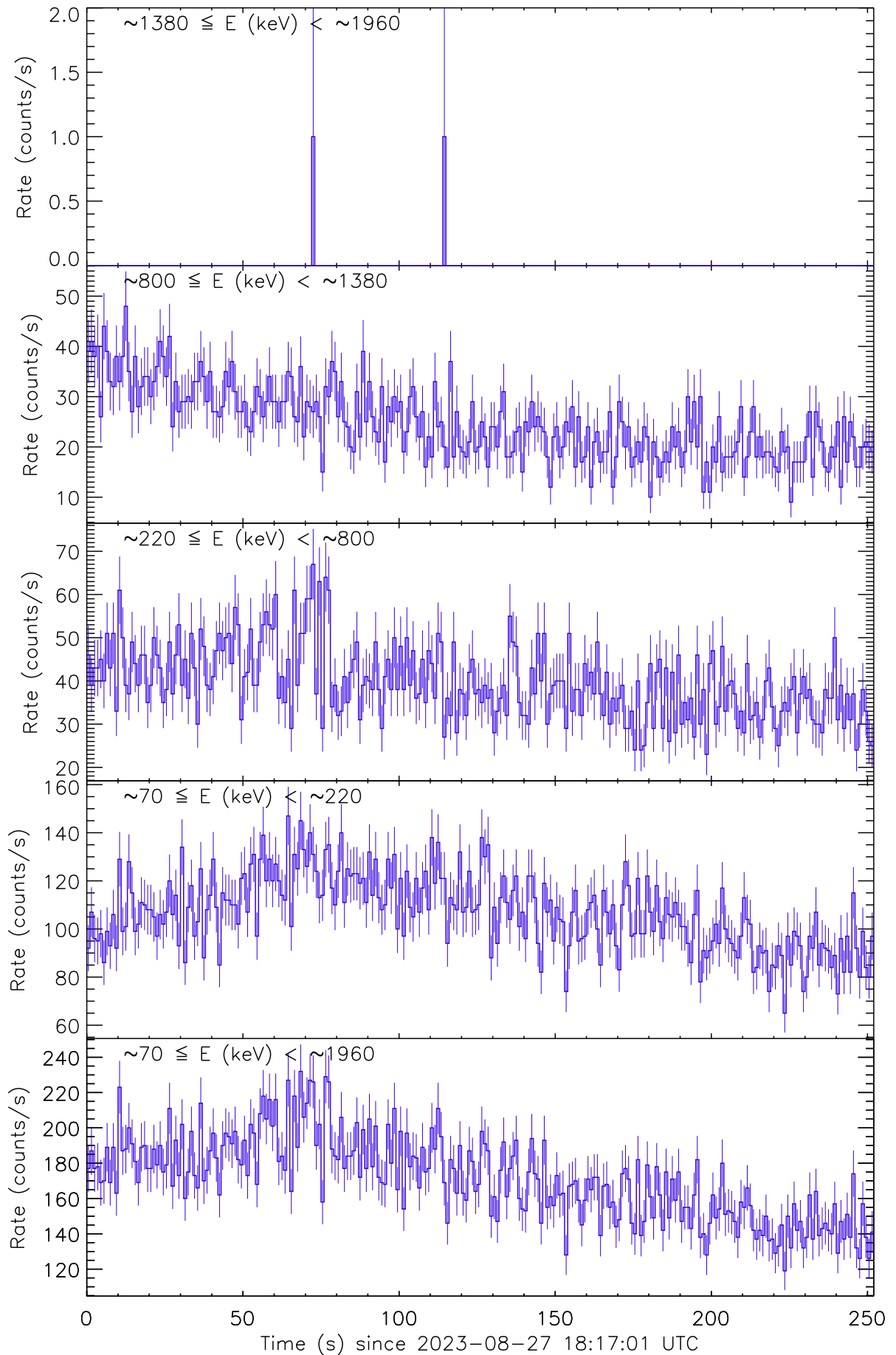
Figure 1: Raw count rate curves of GRB 230827A recorded by the detector unit no. 0.
