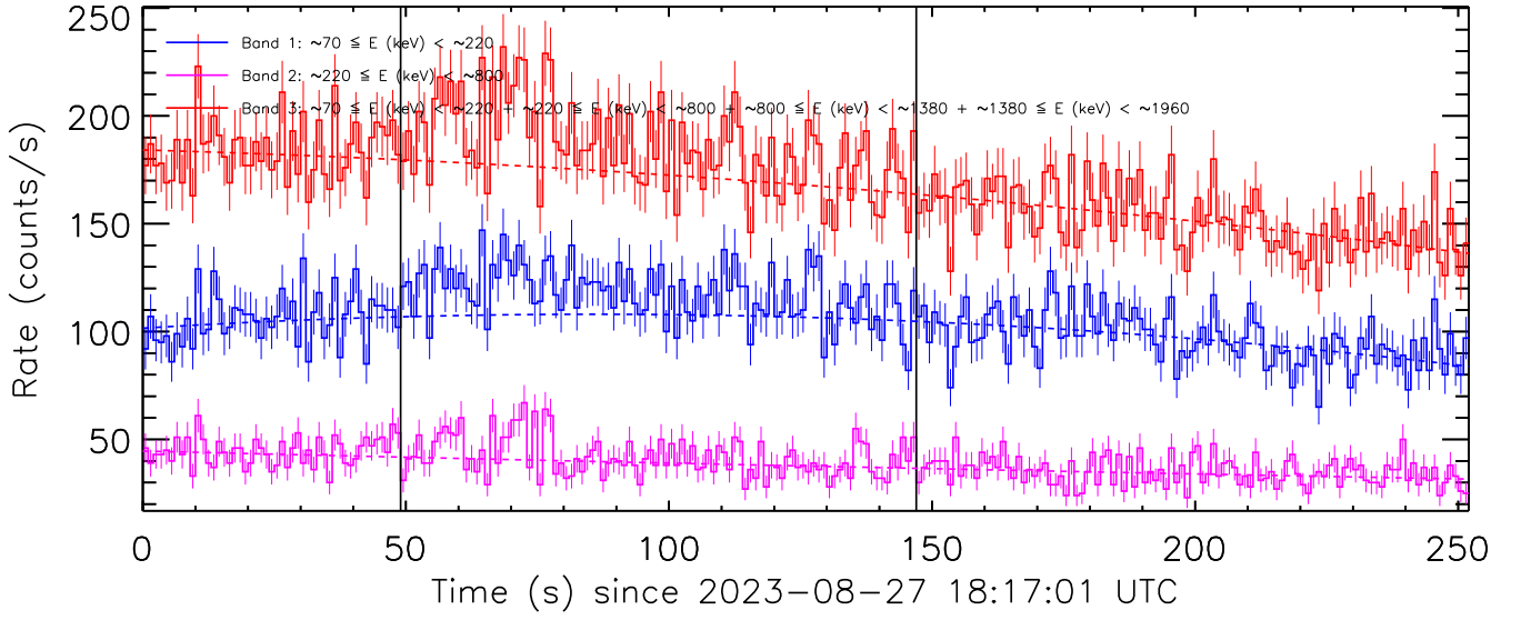
Figure 2: Background fit to the data from the detector unit no. 0 by a second-order polynomial. The pre-burst and post-burst intervals which were used for the background fit are delimited by the vertical solid lines.
