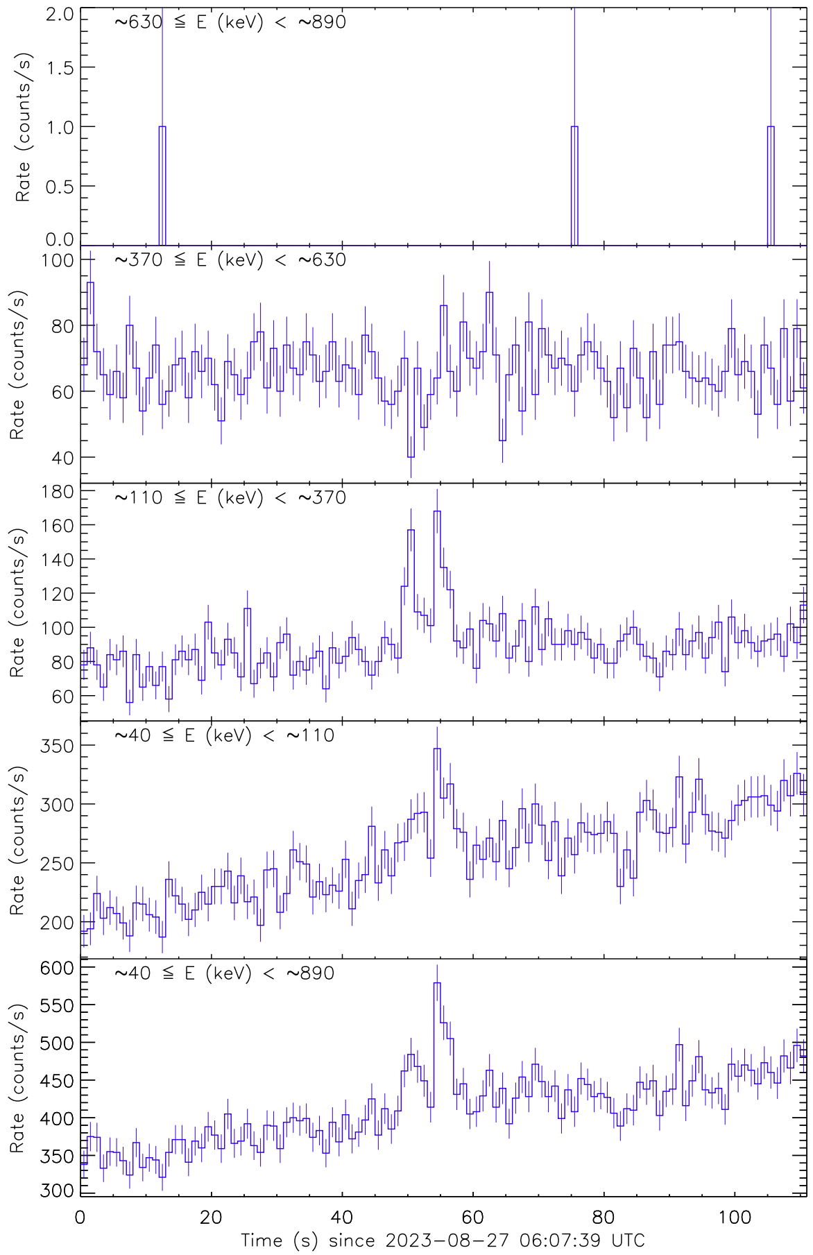
Figure 1: Raw count rate curves of GRB 230827B recorded by the detector unit no. 0.
