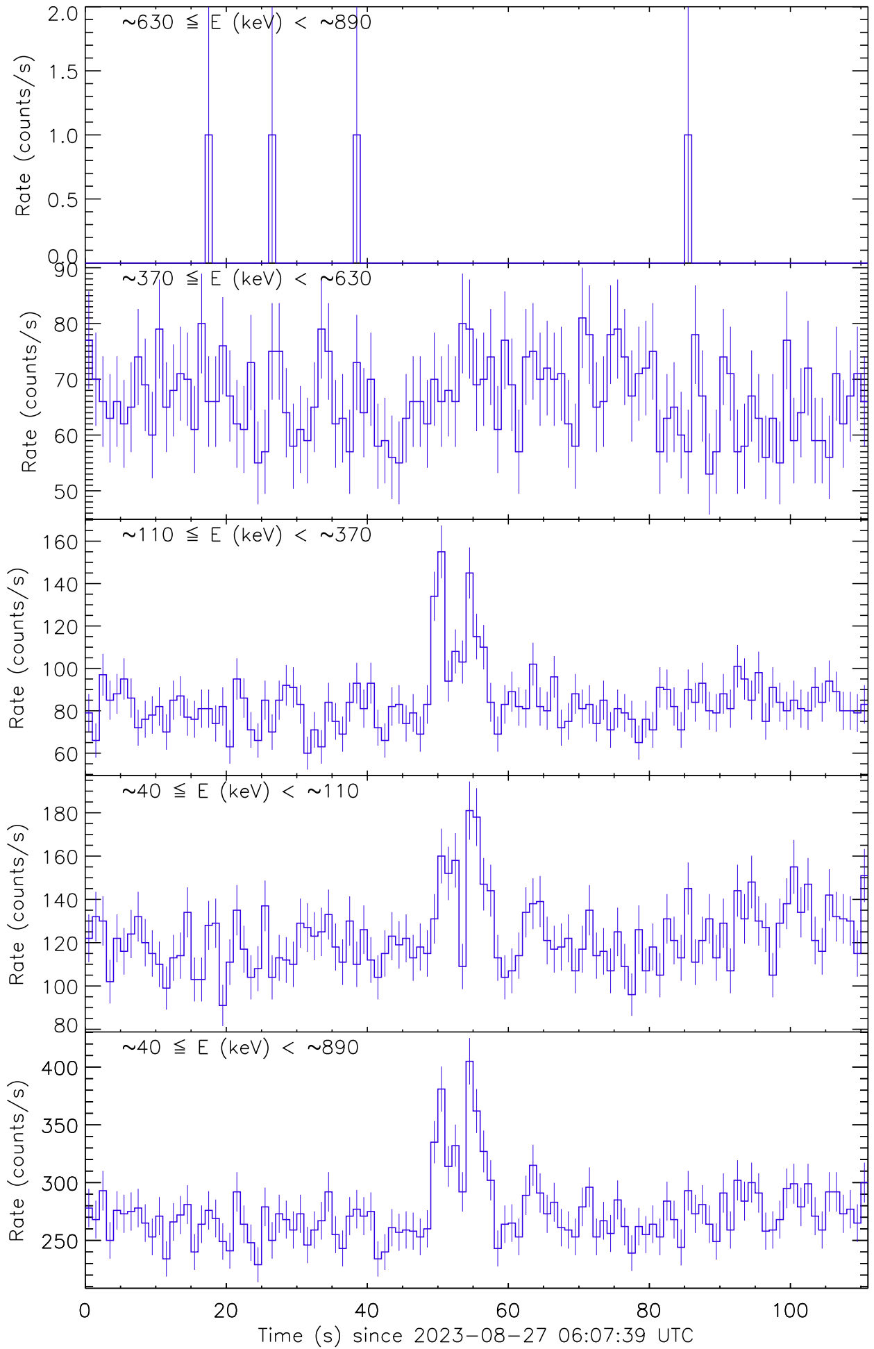
Figure 4: Raw count rate curves of GRB 230827B recorded by the detector unit no. 1.
