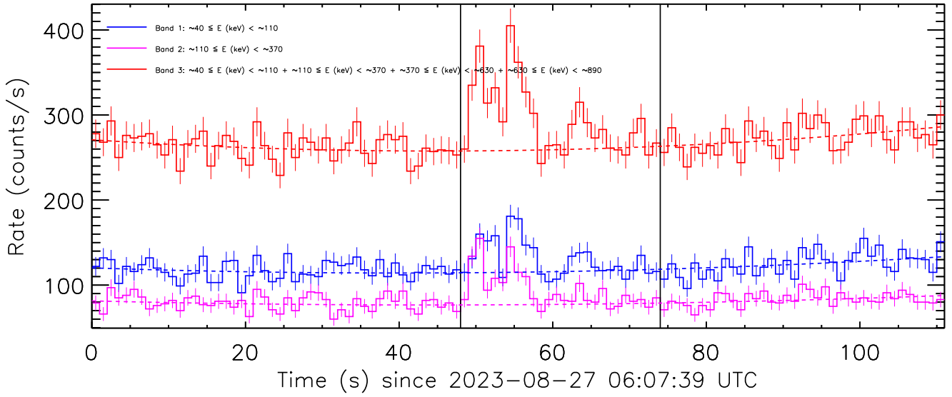
Figure 5: Background fit to the data from the detector unit no. 1 by a second-order polynomial. The pre-burst and post-burst intervals which were used for the background fit are delimited by the vertical solid lines.
