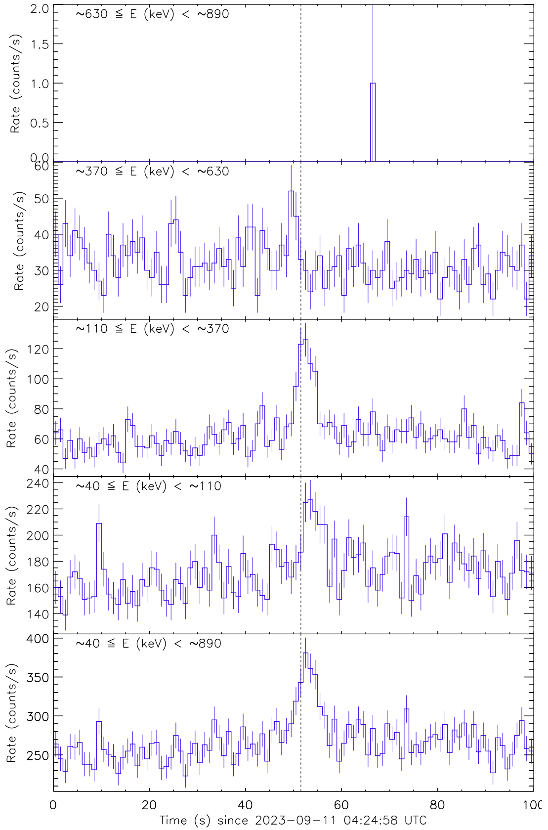
Figure 1: Raw count rate curves of GRB 230911B recorded by the detector unit no. 1. The vertical dashed line marks the trigger time by Fermi/GBM.
