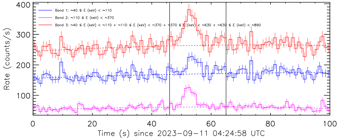
Figure 2: Background fit to the data from the detector unit no. 1 by a second-order polynomial. The pre-burst and post-burst intervals which were used for the background fit are delimited by the vertical solid lines.
