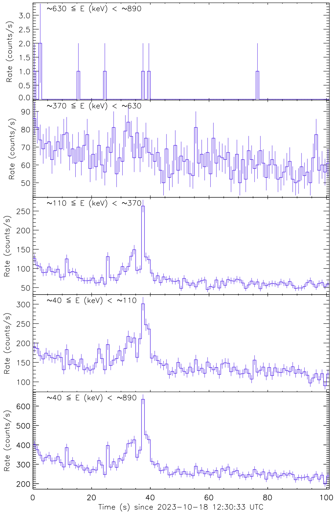
Figure 1: Raw count rate curves of GRB 231018A recorded by the detector unit no. 1.
