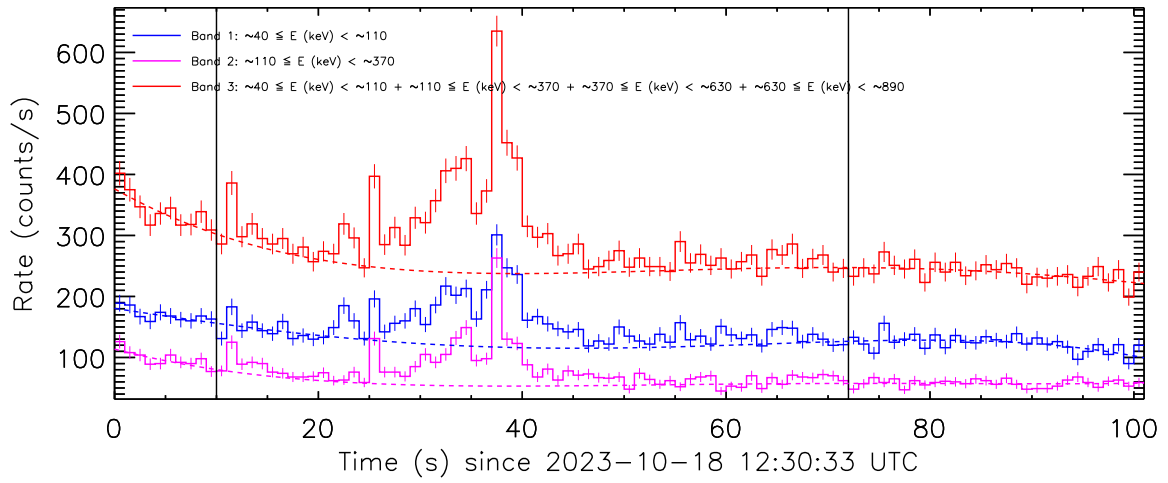
Figure 2: Background fit to the data from the detector unit no. 1 by a fourth-order polynomial. The pre-burst and post-burst intervals which were used for the background fit are delimited by the vertical solid lines.
