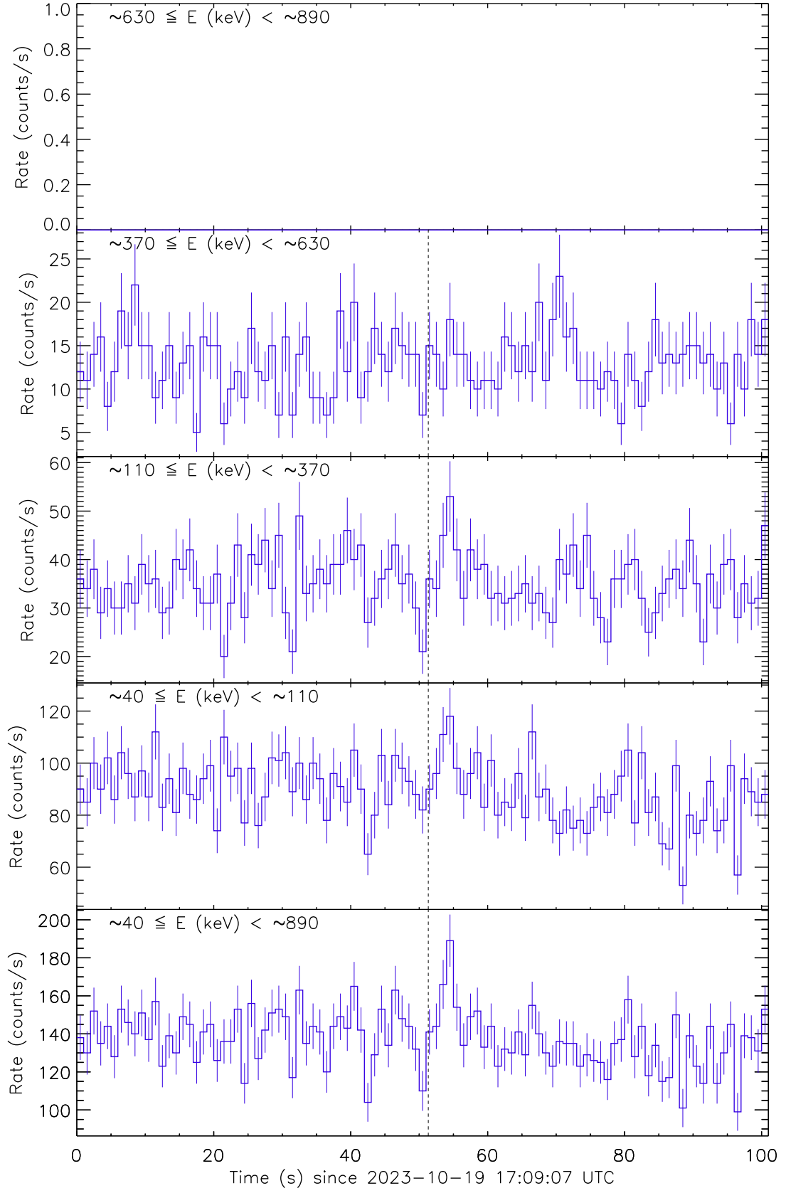
Figure 4: Raw count rate curves of GRB 231019A recorded by the detector unit no. 1. The vertical dashed line marks the trigger time by Fermi/GBM.
