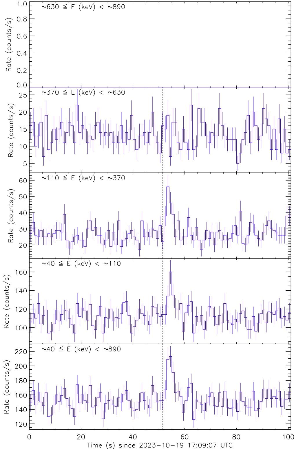
Figure 1: Raw count rate curves of GRB 231019A recorded by the detector unit no. 0. The vertical dashed line marks the trigger time by Fermi/GBM.
