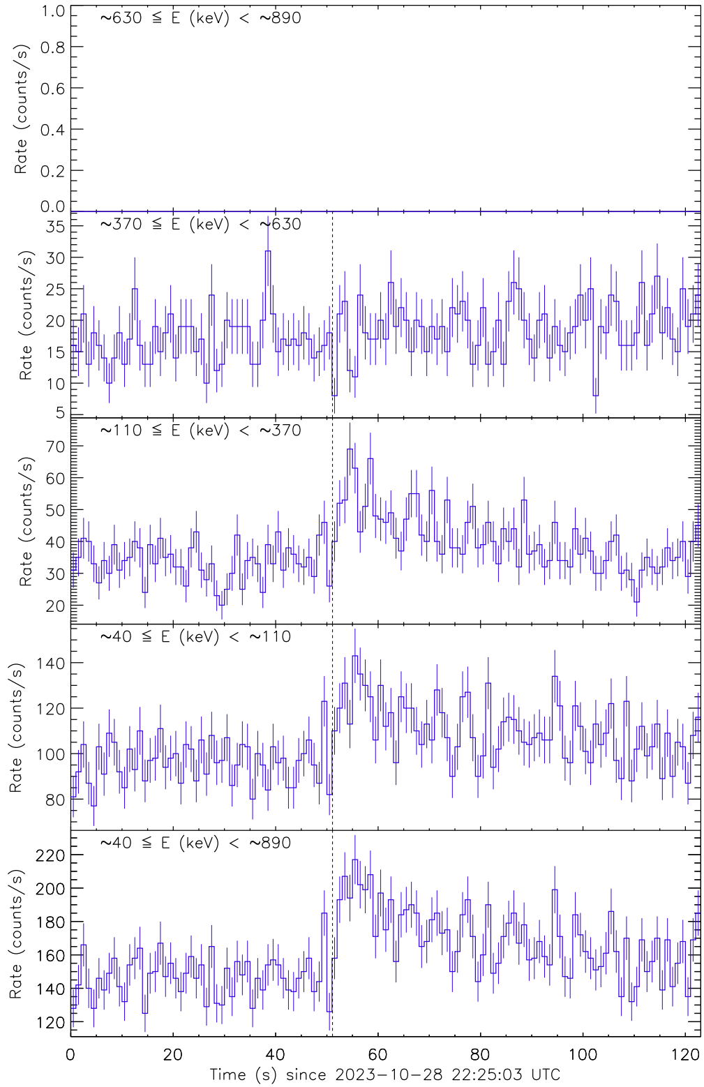
Figure 1: Raw count rate curves of GRB 231028B recorded by the detector unit no. 0. The vertical dashed line marks the trigger time by Fermi/GBM.
