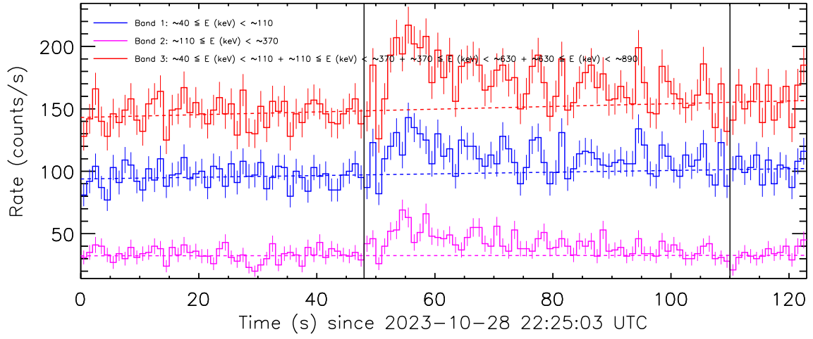
Figure 2: Background fit to the data from the detector unit no. 0 by a linear function. Pre-burst and post-burst intervals which were used for the background fit are delimited by the vertical solid lines.
