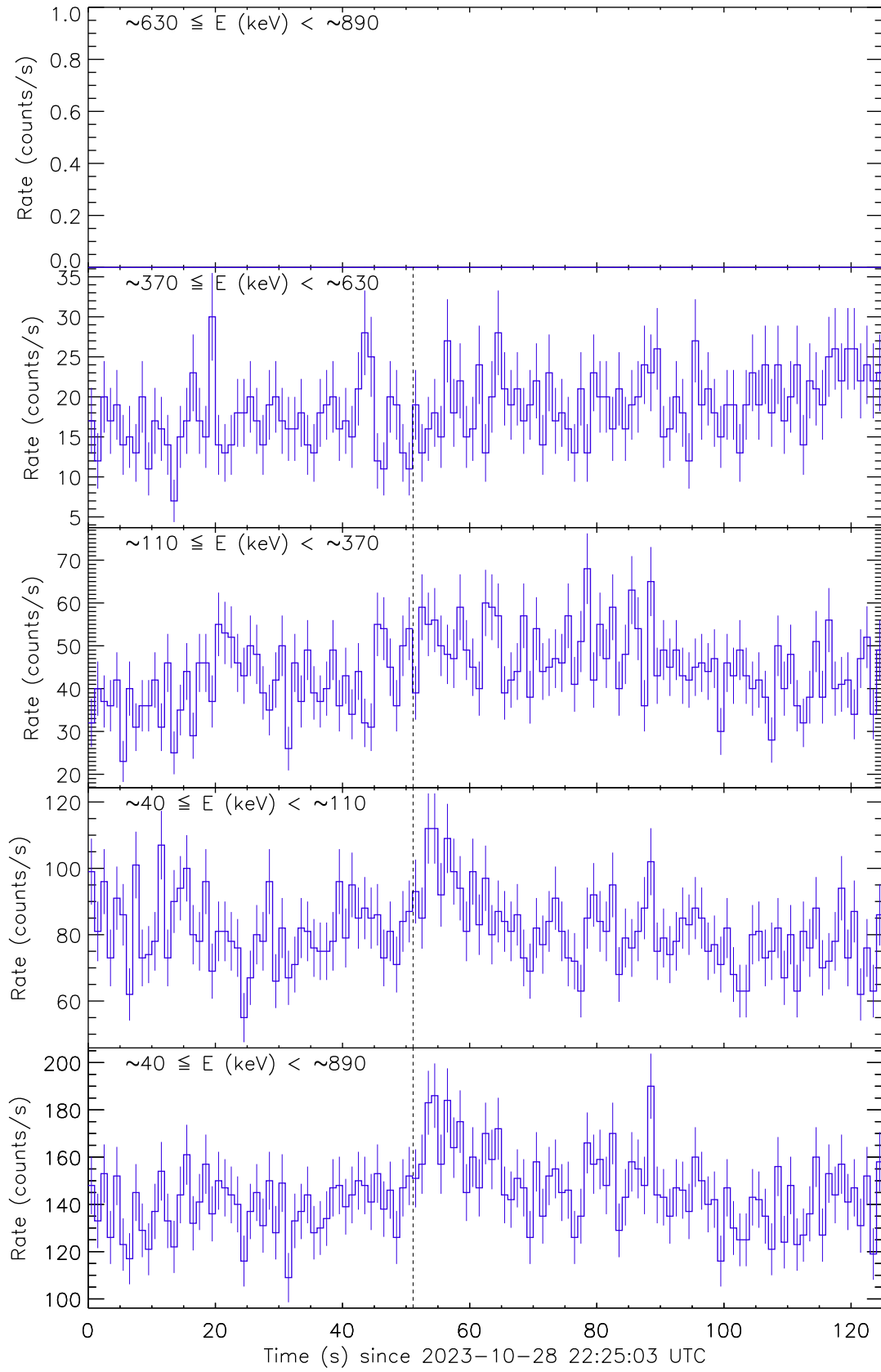
Figure 4: Raw count rate curves of GRB 231028B recorded by the detector unit no. 1. The vertical dashed line marks the trigger time by Fermi/GBM.
