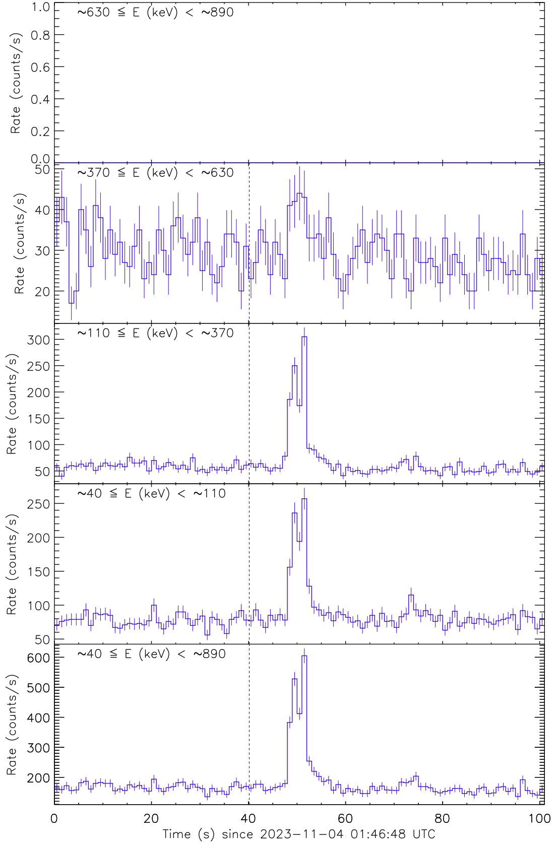
Figure 1: Raw count rate curves of GRB 231104A recorded by the detector unit no. 1. The vertical dashed line marks the trigger time by Fermi/GBM.
