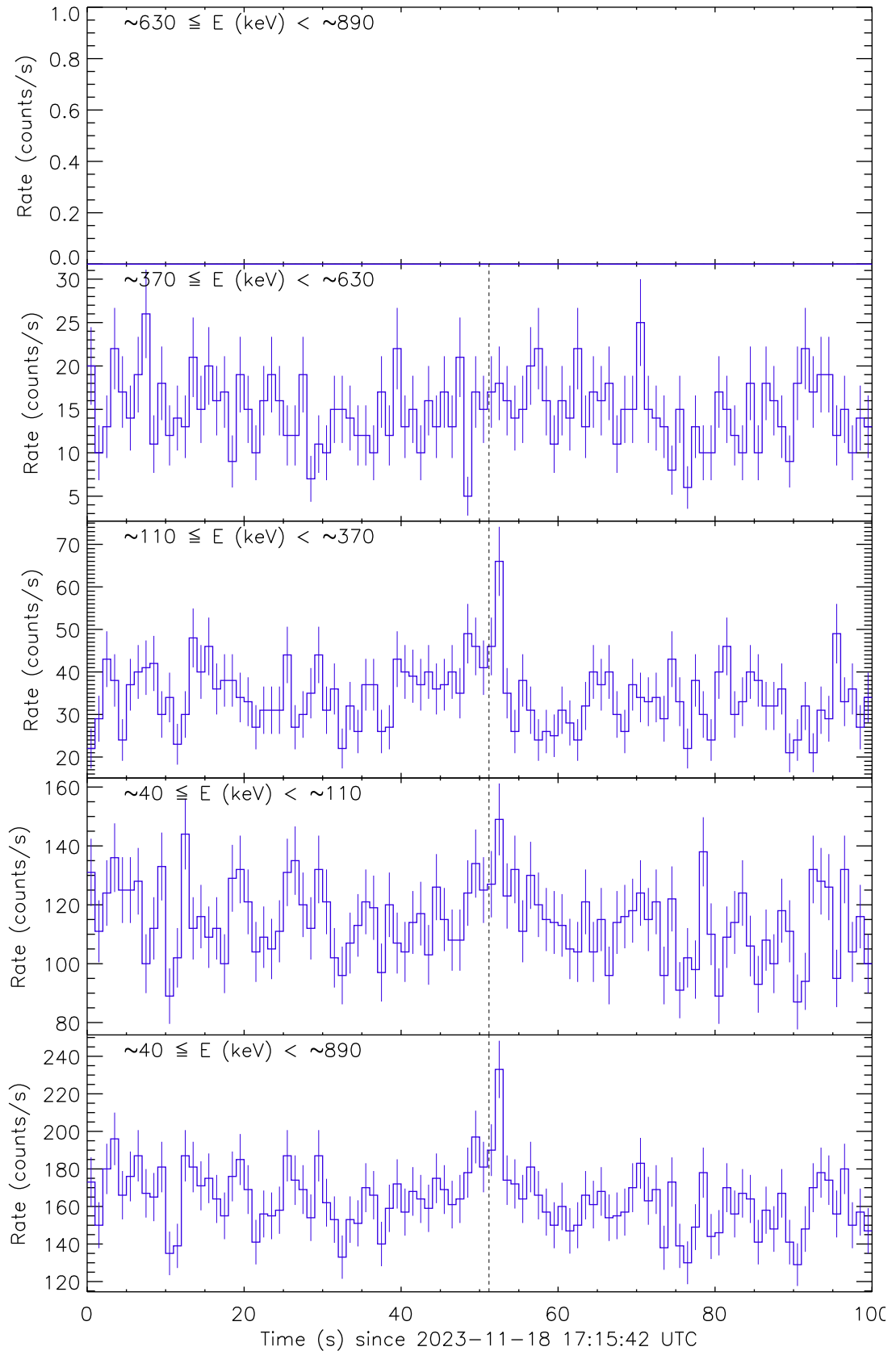
Figure 1: Raw count rate curves of GRB 231118A recorded by the detector unit no. 1. The vertical dashed line marks the trigger time by Swift/BAT.
