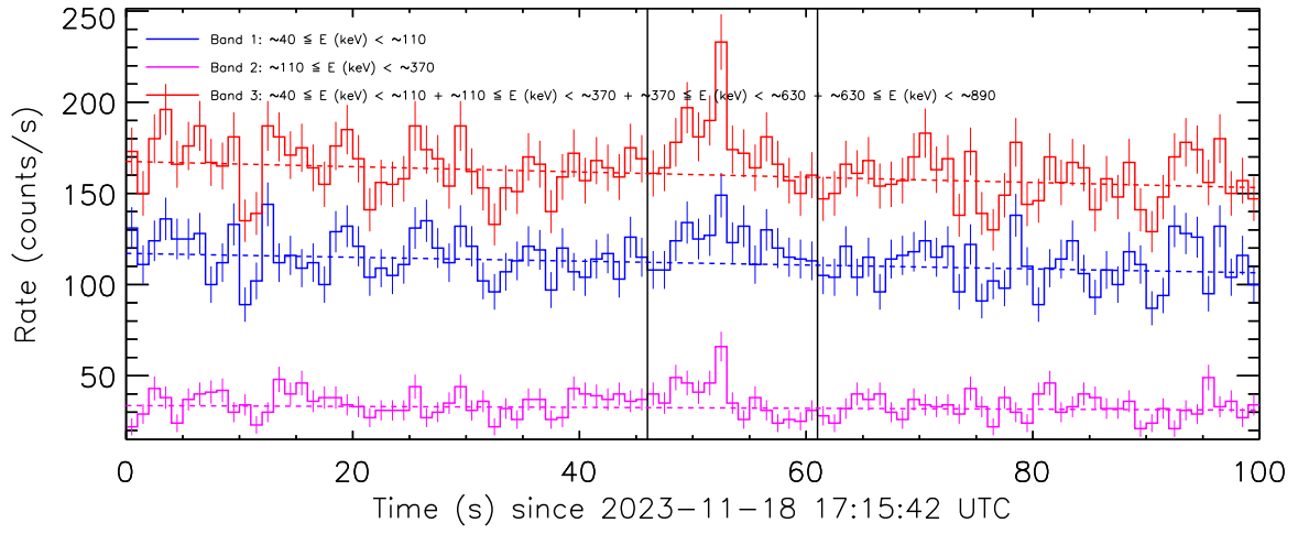
Figure 2: Background fit to the data from the detector unit no. 1 by a linear function. The pre-burst and post-burst intervals which were used for the background fit are delimited by the vertical solid lines.
