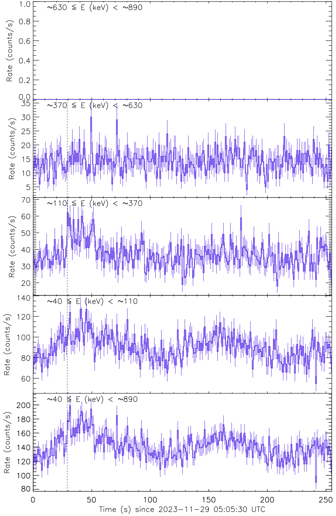
Figure 1: Raw count rate curves of GRB 231129A recorded by the detector unit no. 1. The vertical dashed line marks the trigger time by Swift/BAT.
