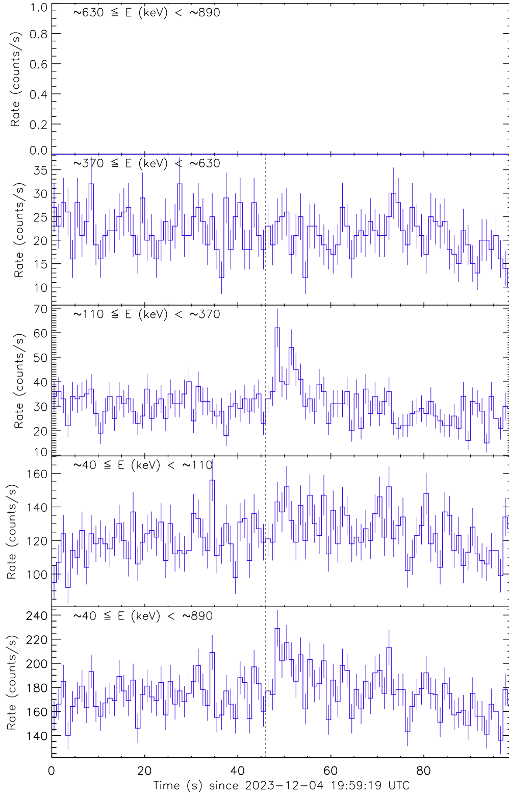
Figure 1: Raw count rate curves of GRB 231204A recorded by the detector unit no. 0. The vertical dashed line marks the trigger time by AstroSat.
