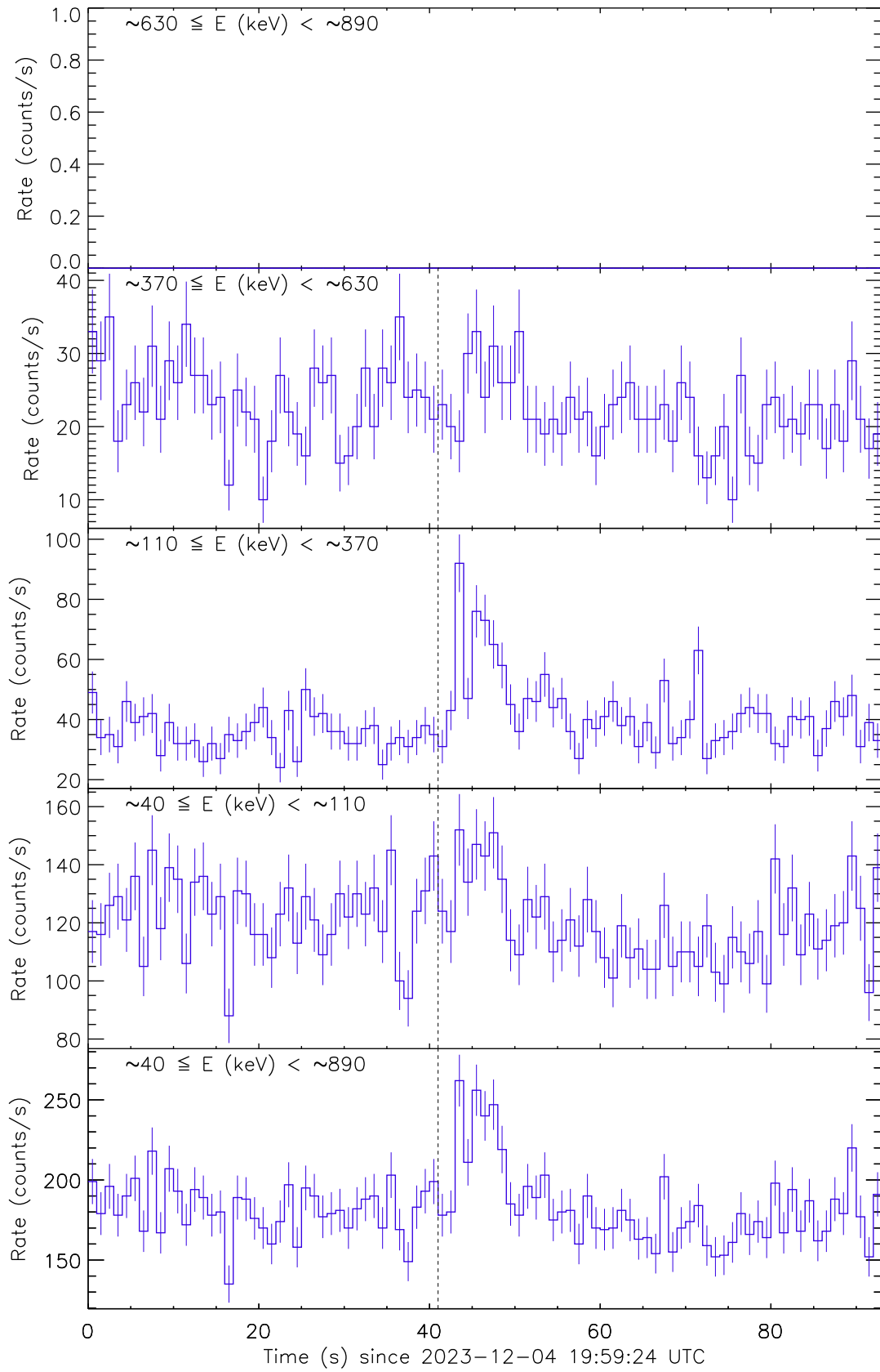
Figure 4: Raw count rate curves of GRB 231204A recorded by the detector unit no. 1. The vertical dashed line marks the trigger time by AstroSat.
