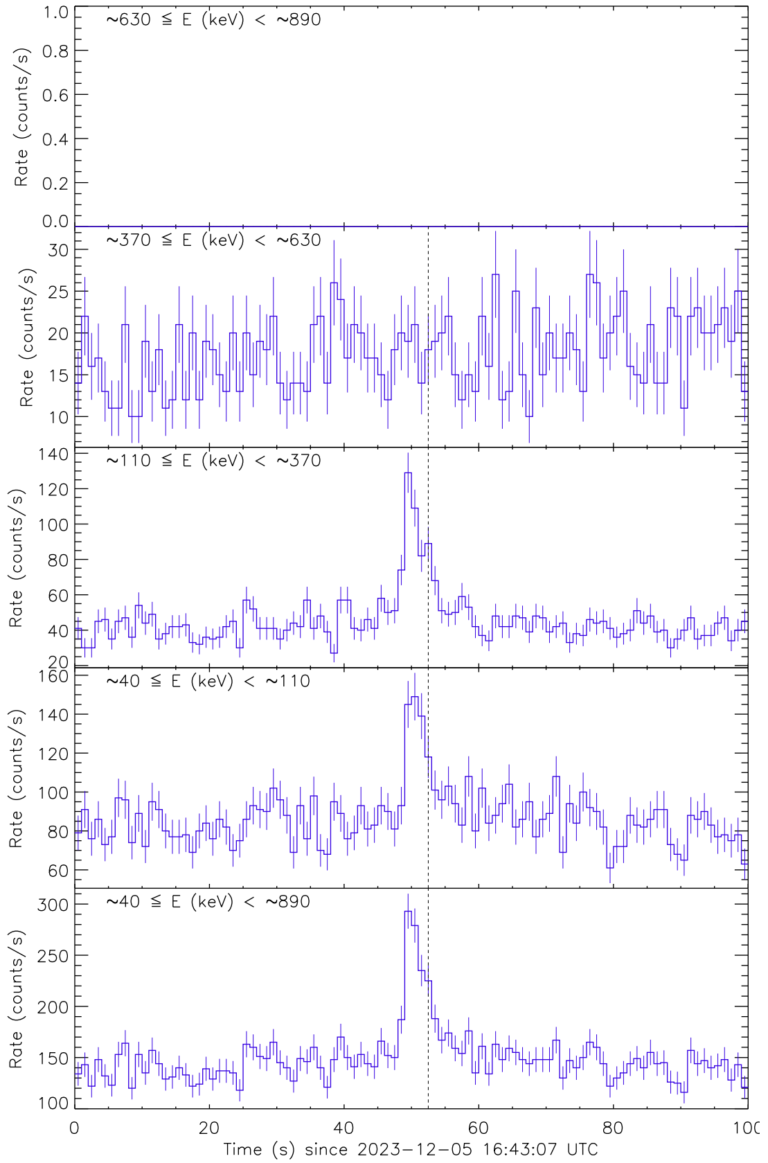
Figure 4: Raw count rate curves of GRB 231205B recorded by the detector unit no. 1. The vertical dashed line marks the trigger time by Swift/BAT.
