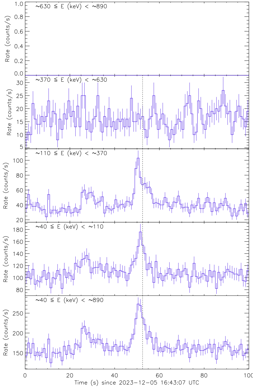
Figure 1: Raw count rate curves of GRB 231205B recorded by the detector unit no. 0. The vertical dashed line marks the trigger time by Swift/BAT.
