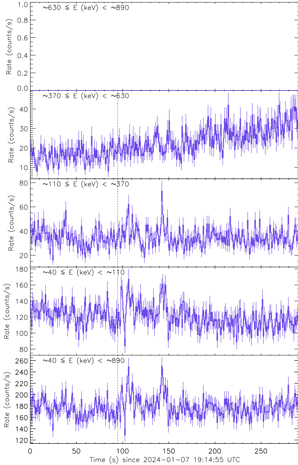
Figure 1: Raw count rate curves of GRB 240107A recorded by the detector unit no. 0. The vertical dashed line marks the trigger time by Fermi/GBM.
