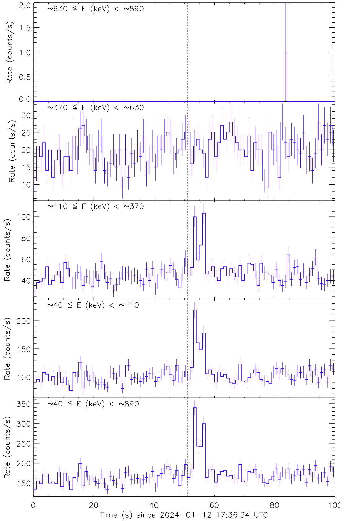
Figure 1: Raw count rate curves of GRB 240112C recorded by the detector unit no. 1. The vertical dashed line marks the trigger time by Fermi/GBM.
