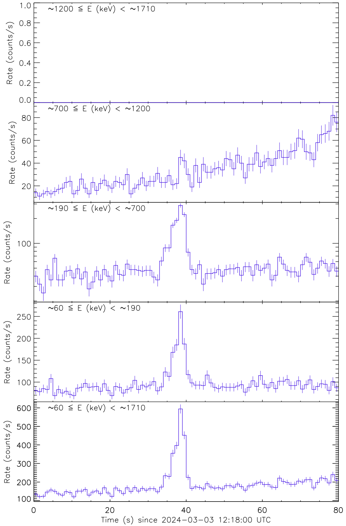
Figure 1: Raw count rate curves of GRB 240303B recorded by the detector unit no. 1.
