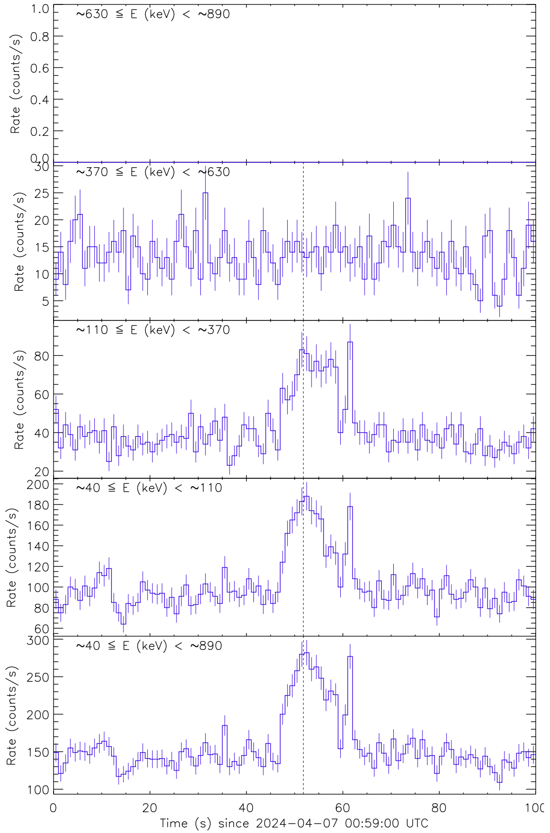
Figure 1: Raw count rate curves of GRB 240407A recorded by the detector unit no. 1. The vertical dashed line marks the trigger time by Fermi/GBM.
