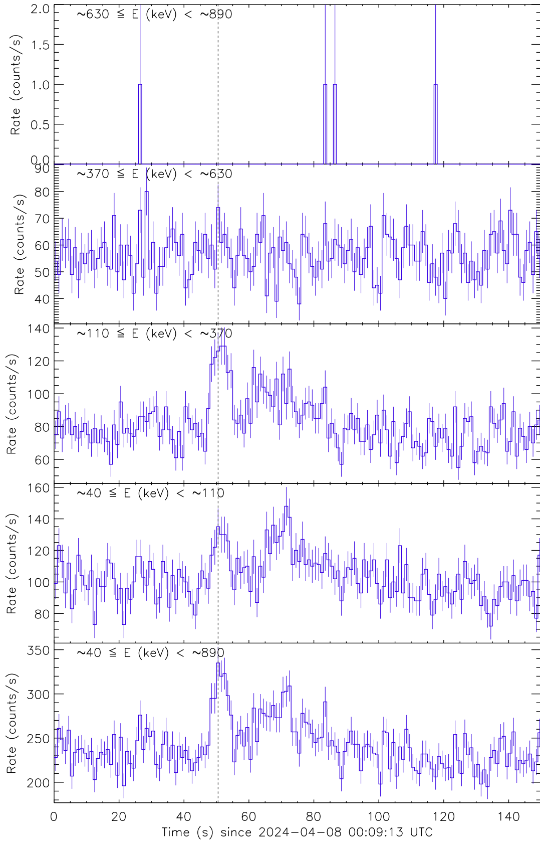
Figure 1: Raw count rate curves of GRB 240408B recorded by the detector unit no. 1. The vertical dashed line marks the trigger time by AstroSat/CZTI.
