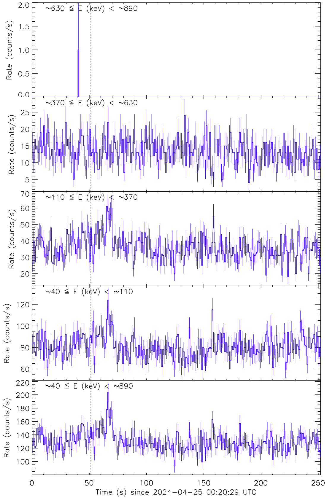
Figure 1: Raw count rate curves of GRB 240425A recorded by the detector unit no. 1. The vertical dashed line marks the trigger time by Fermi/GBM.
