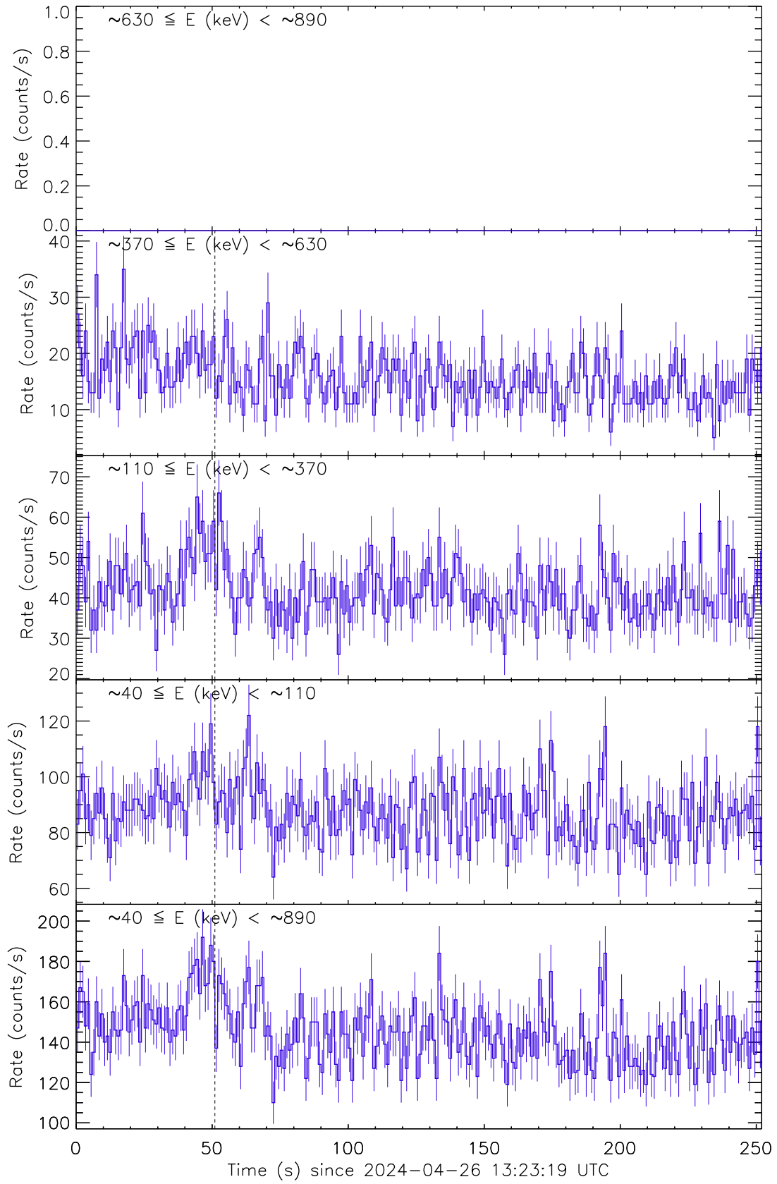
Figure 1: Raw count rate curves of GRB 240426A recorded by the detector unit no. 1. The vertical dashed line marks the trigger time by AstroSat/CZTI.
