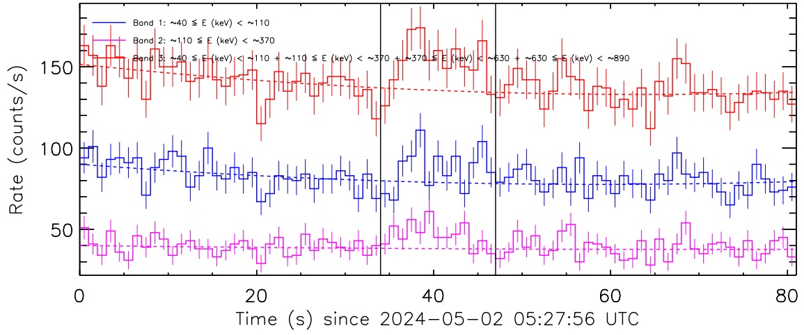
Figure 2: Background fit to the data from the detector unit no. 1 by a second-order polynomial. The pre-burst and post-burst intervals which were used for the background fit are delimited by the vertical solid lines.
