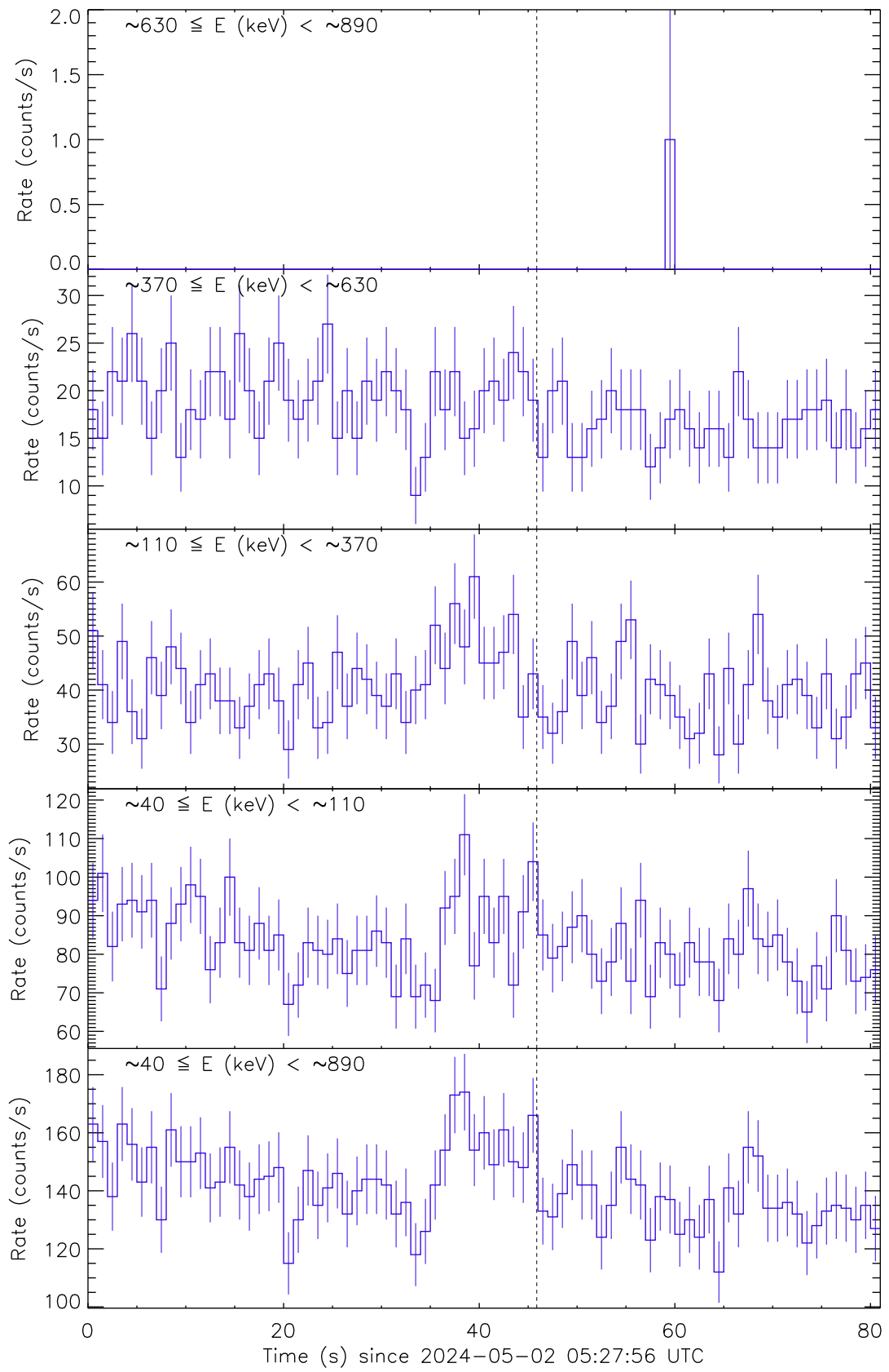
Figure 1: Raw count rate curves of GRB 240502A recorded by the detector unit no. 1. The vertical dashed line marks the trigger time by Fermi/GBM.
