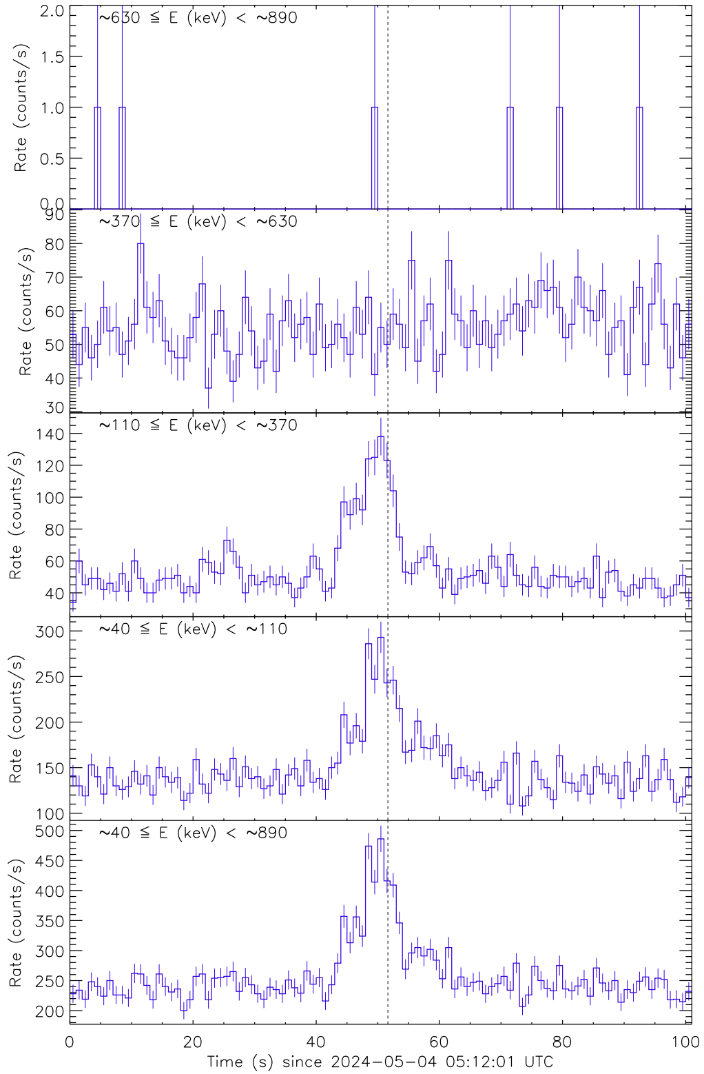
Figure 1: Raw count rate curves of GRB 240504A recorded by the detector unit no. 0. The vertical dashed line marks the trigger time by Fermi/GBM.
