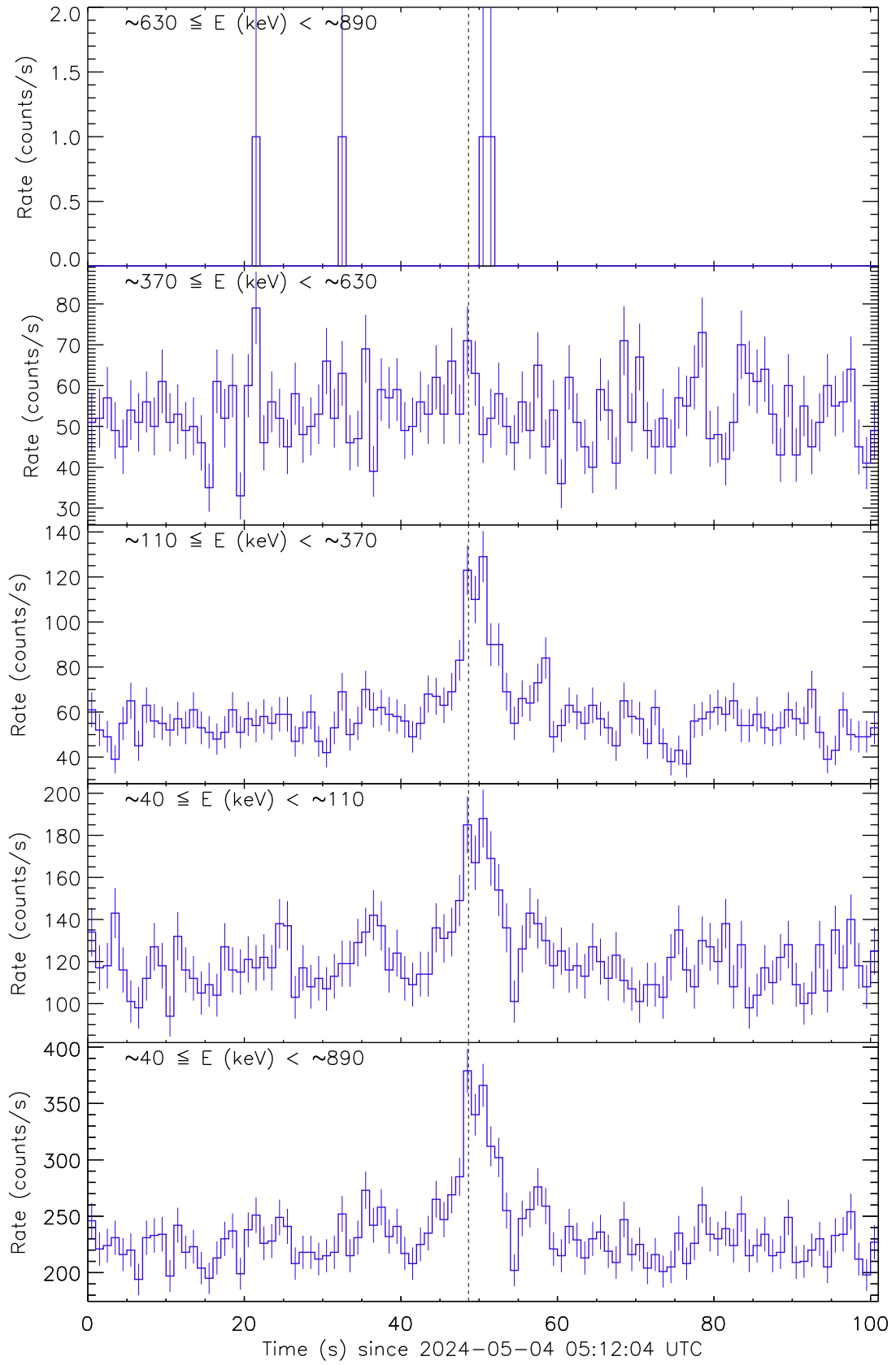
Figure 4: Raw count rate curves of GRB 240504A recorded by the detector unit no. 1. The vertical dashed line marks the trigger time by Fermi/GBM.
