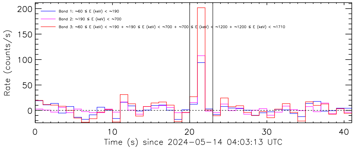
Figure 3: Background-subtracted count rate curves from the detector unit no. 1.
