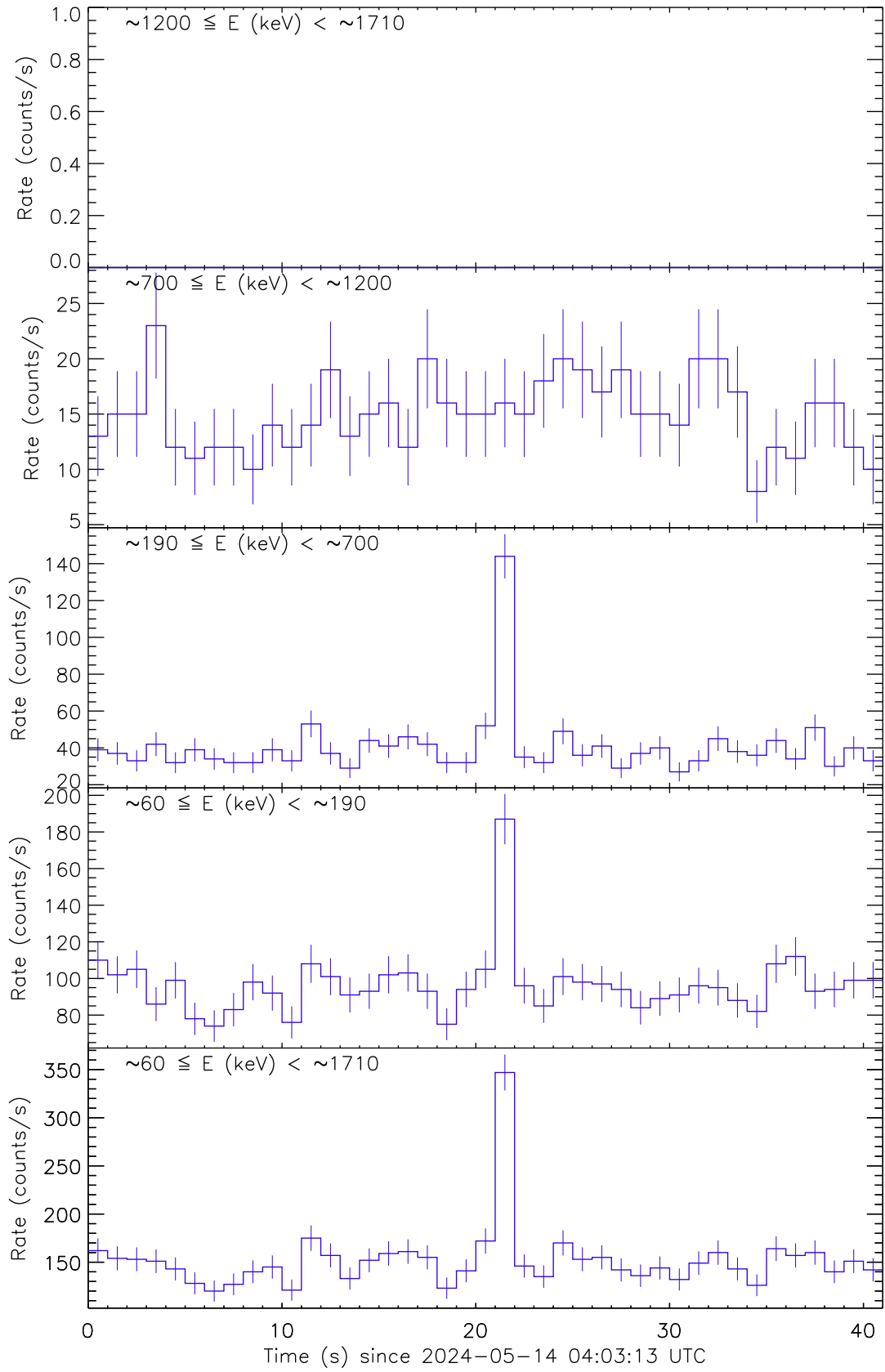
Figure 1: Raw count rate curves of GRB 240514B recorded by the detector unit no. 1.
