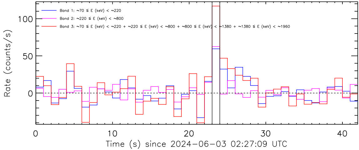
Figure 3: Background-subtracted count rate curves from the detector unit no. 0.
