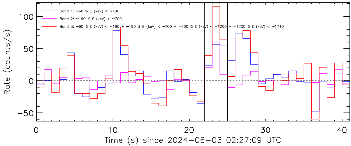
Figure 6: Background-subtracted count rate curves from the detector unit no. 1.
