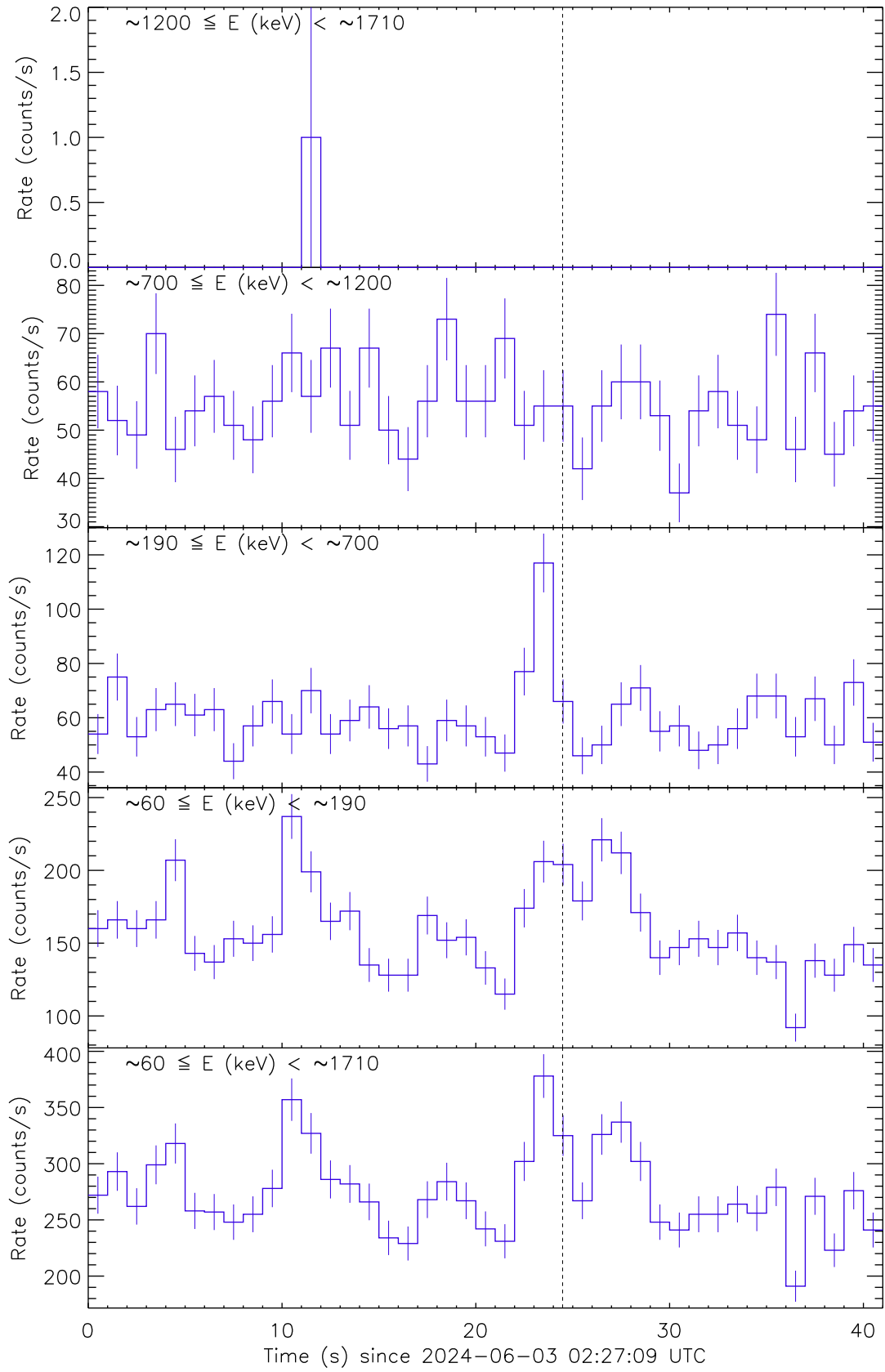
Figure 4: Raw count rate curves of GRB 240603A recorded by the detector unit no. 1. The vertical dashed line marks the trigger time by Fermi/GBM.
