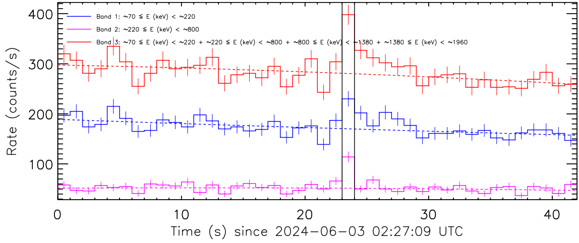
Figure 2: Background fit to the data from the detector unit no. 0 by a second-order polynomial. Pre-burst and post-burst intervals which were used for the background fit are delimited by the vertical solid lines.
