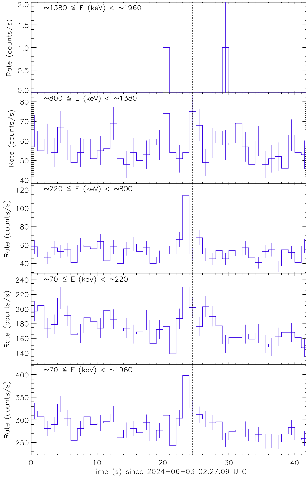
Figure 1: Raw count rate curves of GRB 240603A recorded by the detector unit no. 0. The vertical dashed line marks the trigger time by Fermi/GBM.
