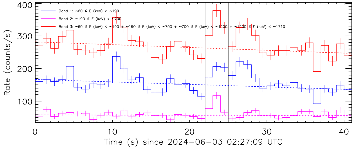
Figure 5: Background fit to the data from the detector unit no. 1 by a linear function. The pre-burst and post-burst intervals which were used for the background fit are delimited by the vertical solid lines.
