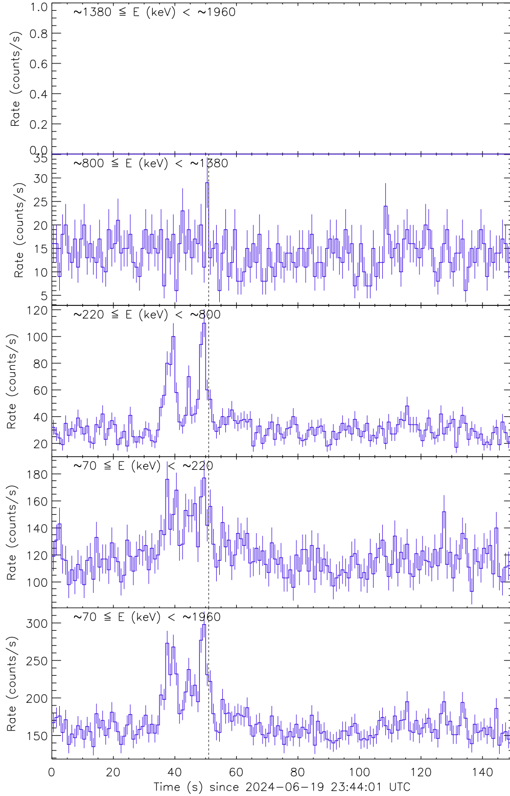
Figure 1: Raw count rate curves of GRB 240619C recorded by the detector unit no. 0. The vertical dashed line marks the trigger time by AstroSat/CZTI.
