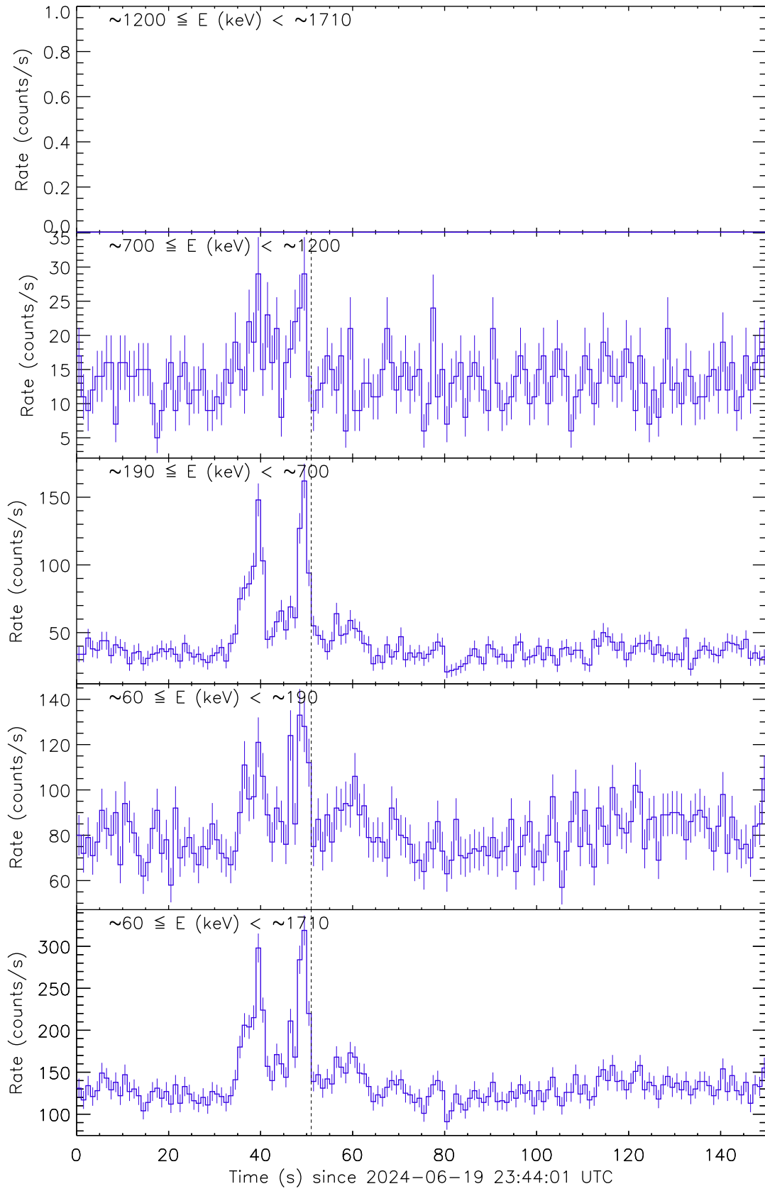
Figure 4: Raw count rate curves of GRB 240619C recorded by the detector unit no. 1. The vertical dashed line marks the trigger time by AstroSat/CZTI.
