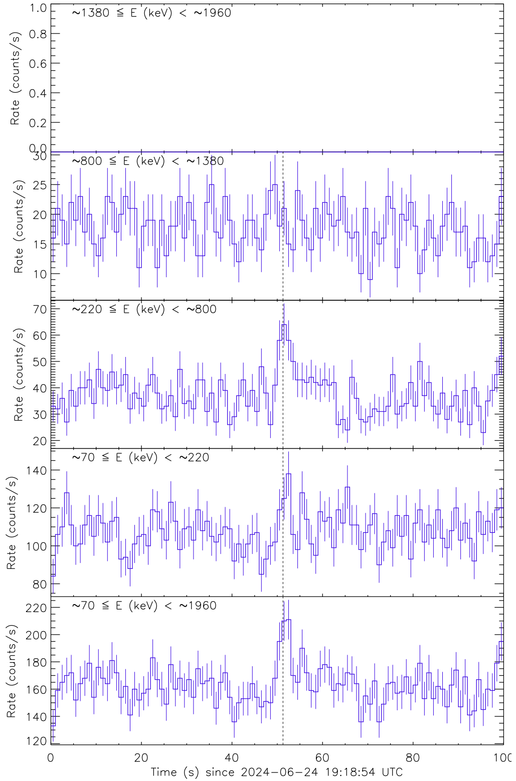
Figure 1: Raw count rate curves of GRB 240624B recorded by the detector unit no. 0. The vertical dashed line marks the trigger time by Fermi/GBM.
