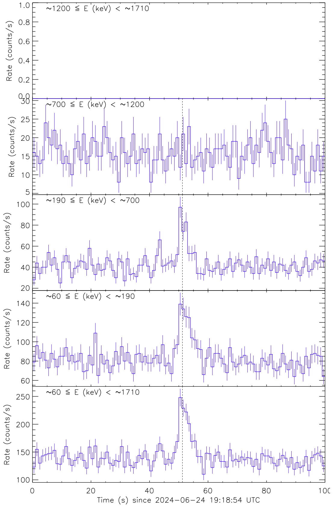
Figure 4: Raw count rate curves of GRB 240624B recorded by the detector unit no. 1. The vertical dashed line marks the trigger time by Fermi/GBM.
