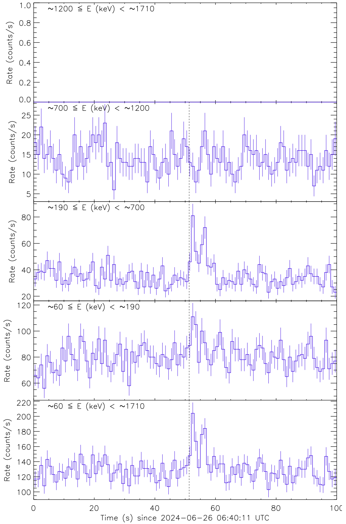
Figure 1: Raw count rate curves of GRB 240626B recorded by the detector unit no. 1. The vertical dashed line marks the trigger time by INTEGRAL/SPI-ACS.
