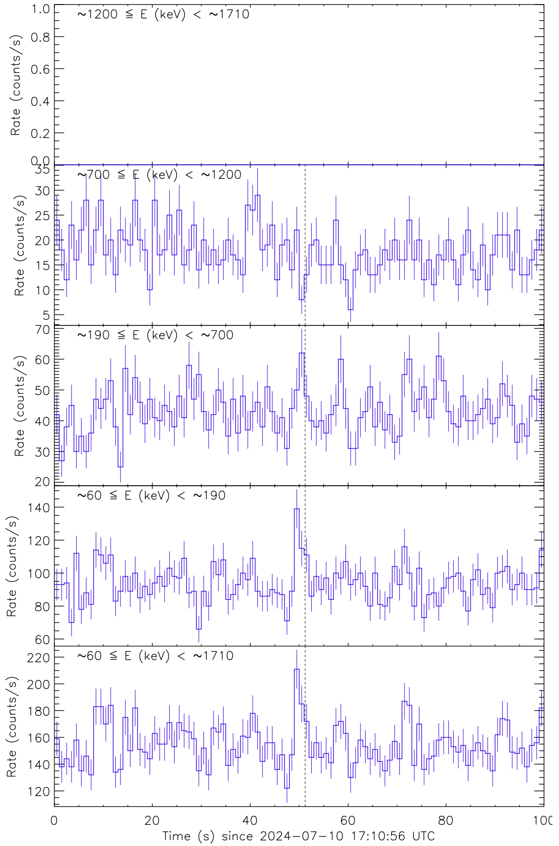
Figure 1: Raw count rate curves of GRB 240710A recorded by the detector unit no. 1. The vertical dashed line marks the trigger time by Fermi/GBM.
