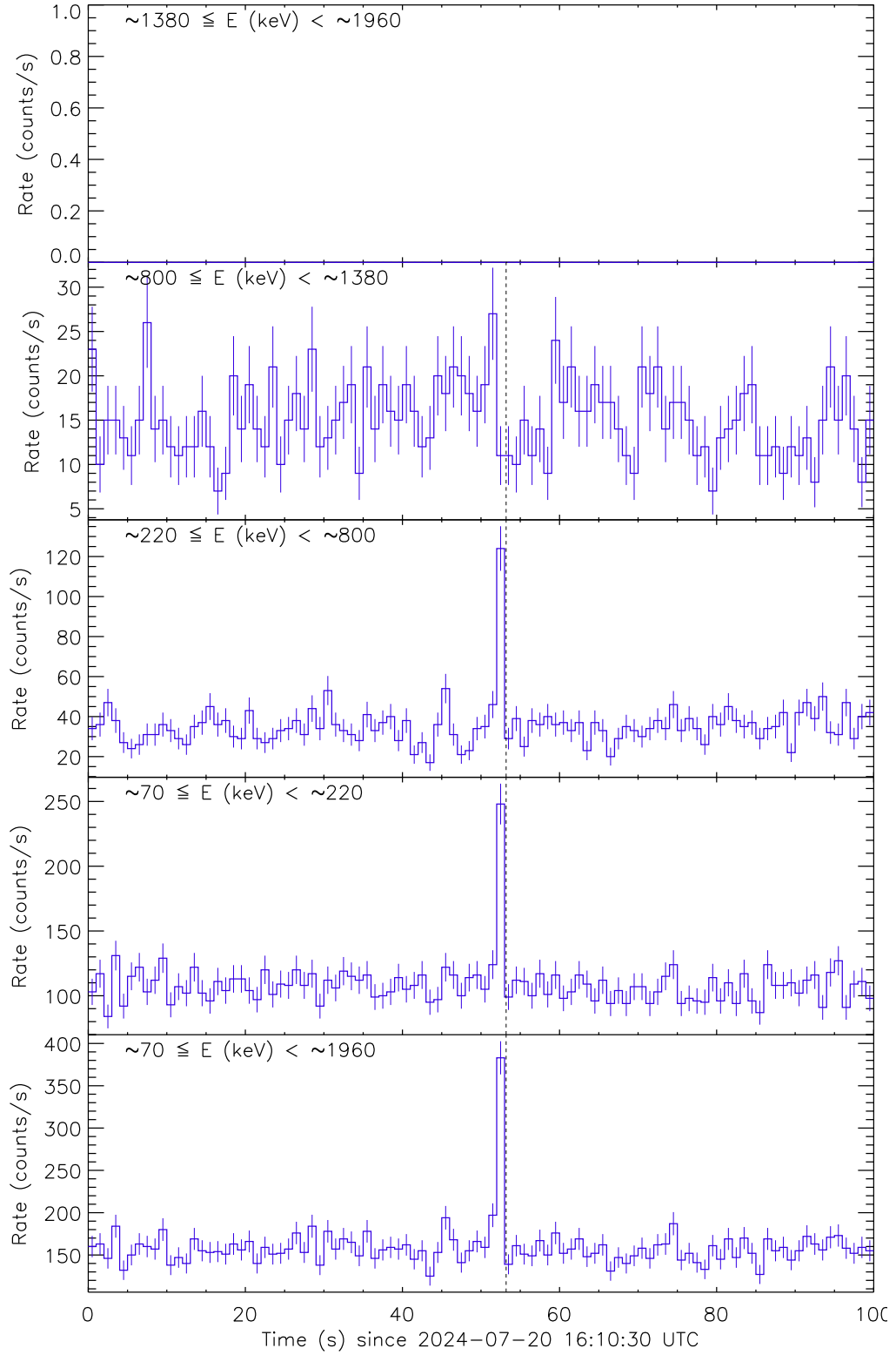
Figure 1: Raw count rate curves of GRB 240720B recorded by the detector unit no. 0. The vertical dashed line marks the trigger time by SVOM/GRM.
