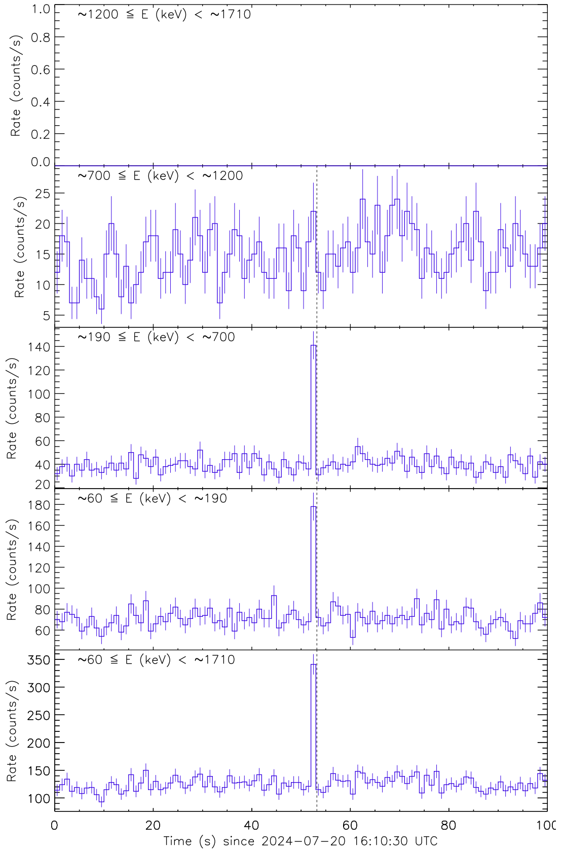
Figure 4: Raw count rate curves of GRB 240720B recorded by the detector unit no. 1. The vertical dashed line marks the trigger time by SVOM/GRM.
