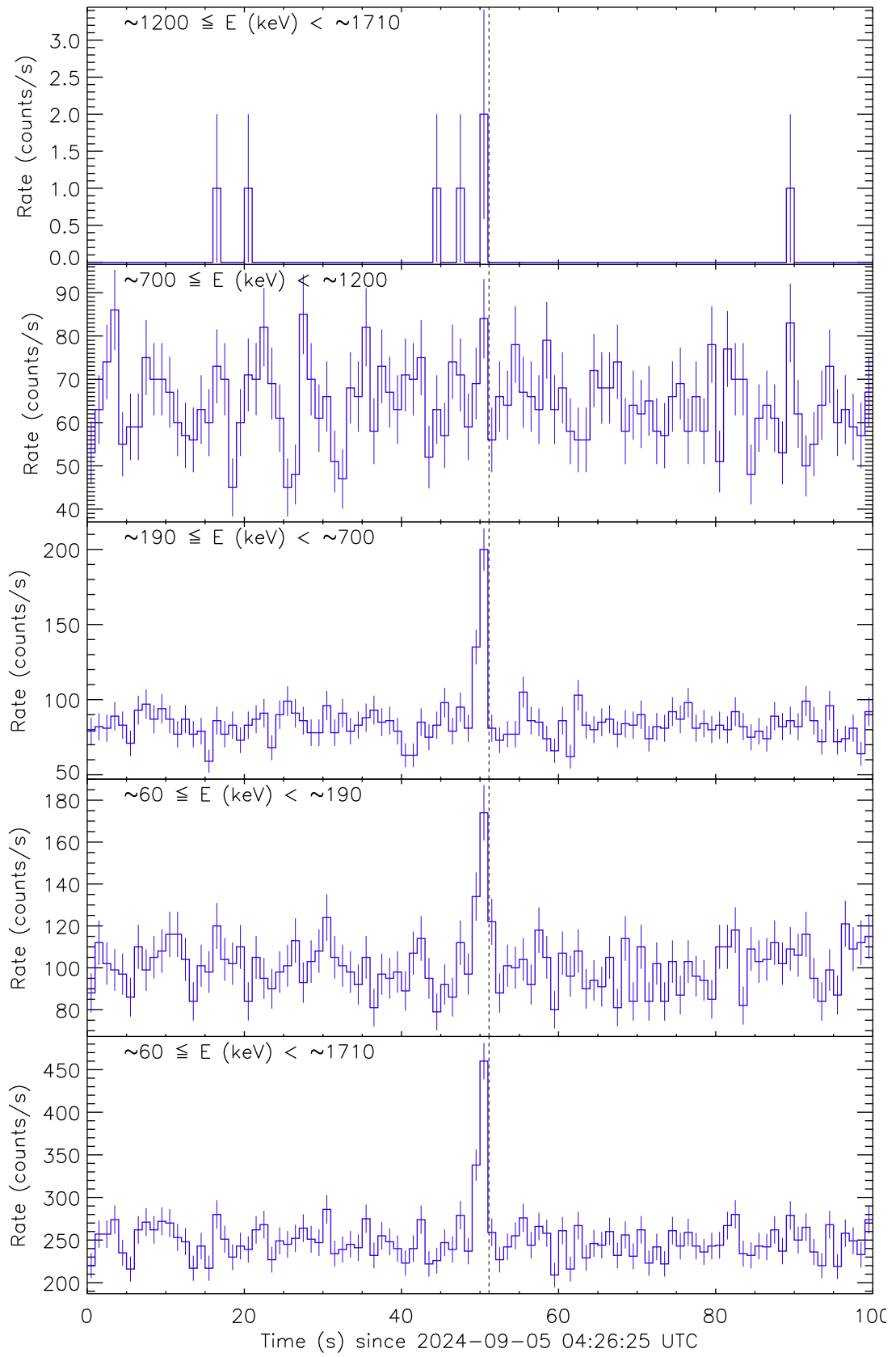
Figure 1: Raw count rate curves of GRB 240905B recorded by the detector unit no. 1. The vertical dashed line marks the trigger time by Fermi/GBM.
