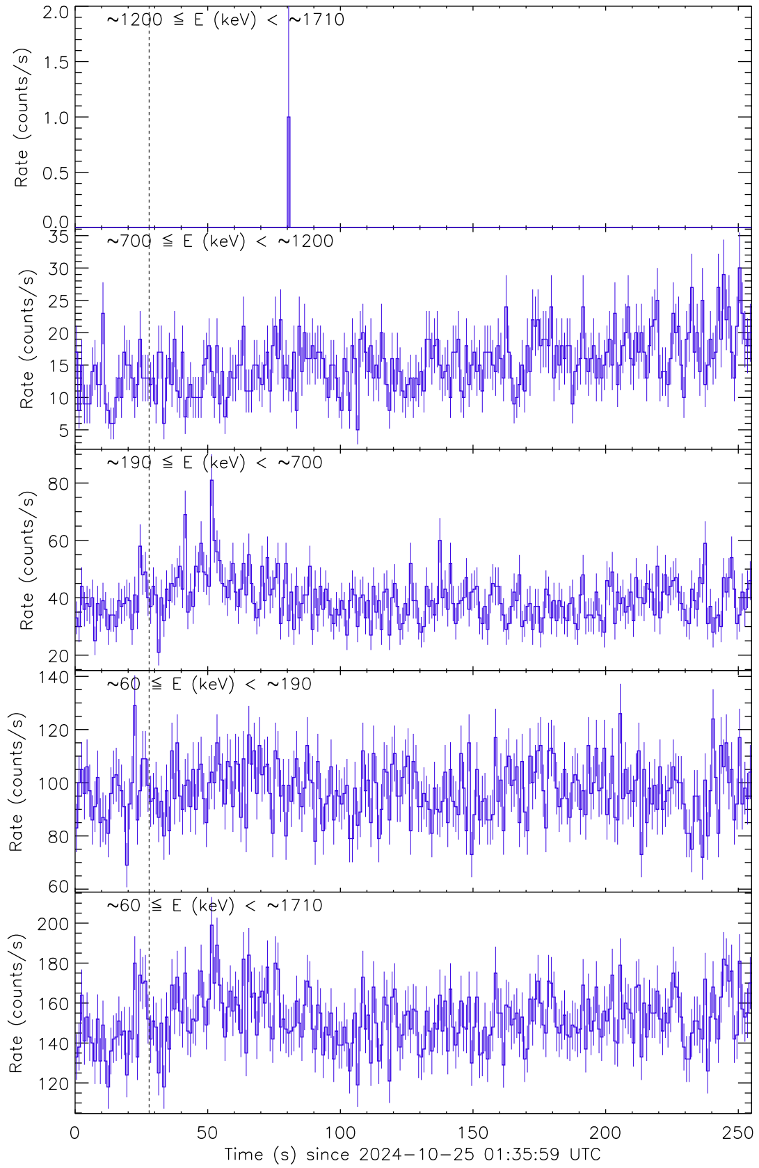
Figure 1: Raw count rate curves of GRB 241025A recorded by the detector unit no. 1. The vertical dashed line marks the trigger time by Fermi/GBM.
