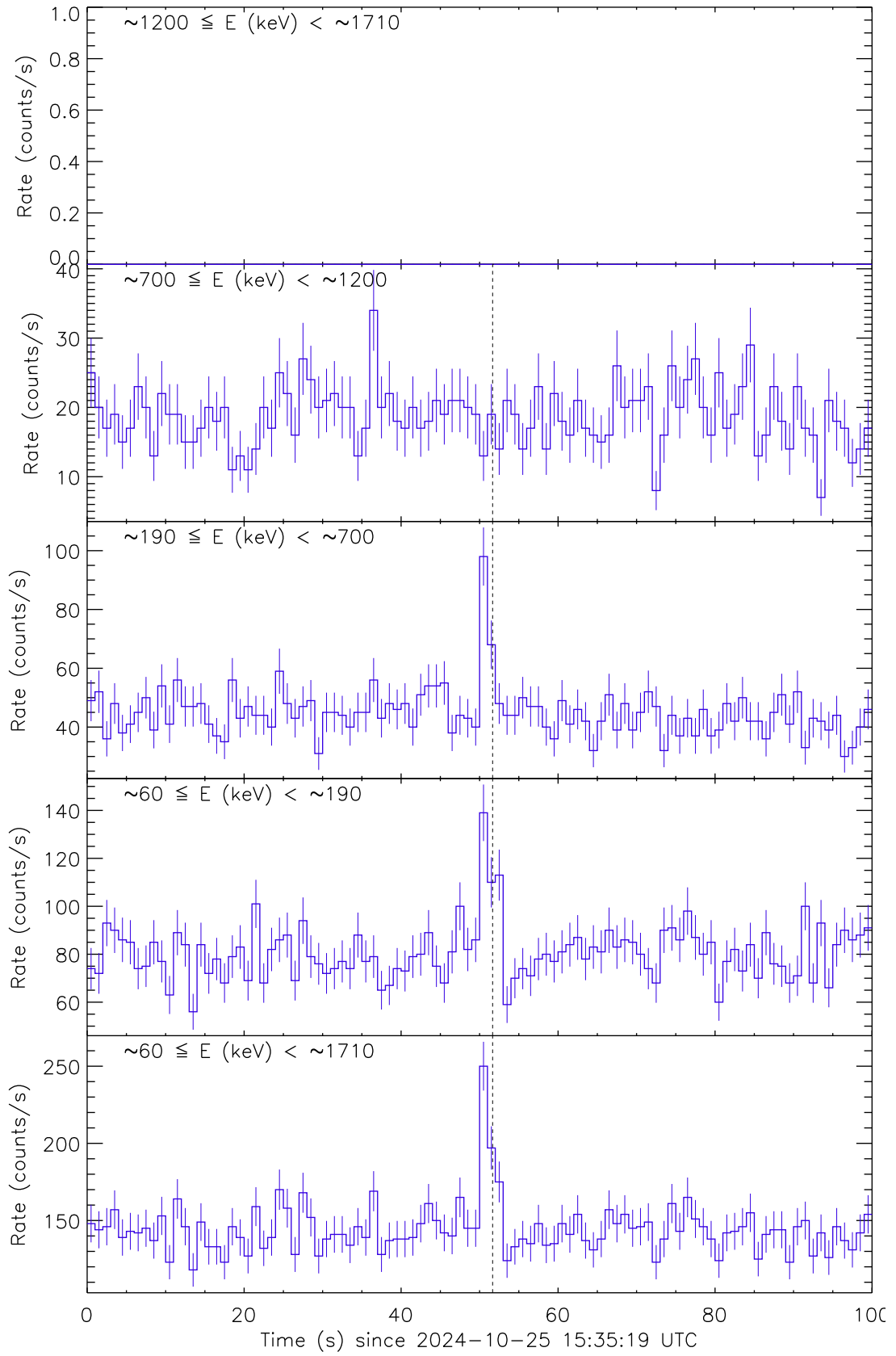
Figure 1: Raw count rate curves of GRB 241025C recorded by the detector unit no. 1. The vertical dashed line marks the trigger time by Fermi/GBM.
