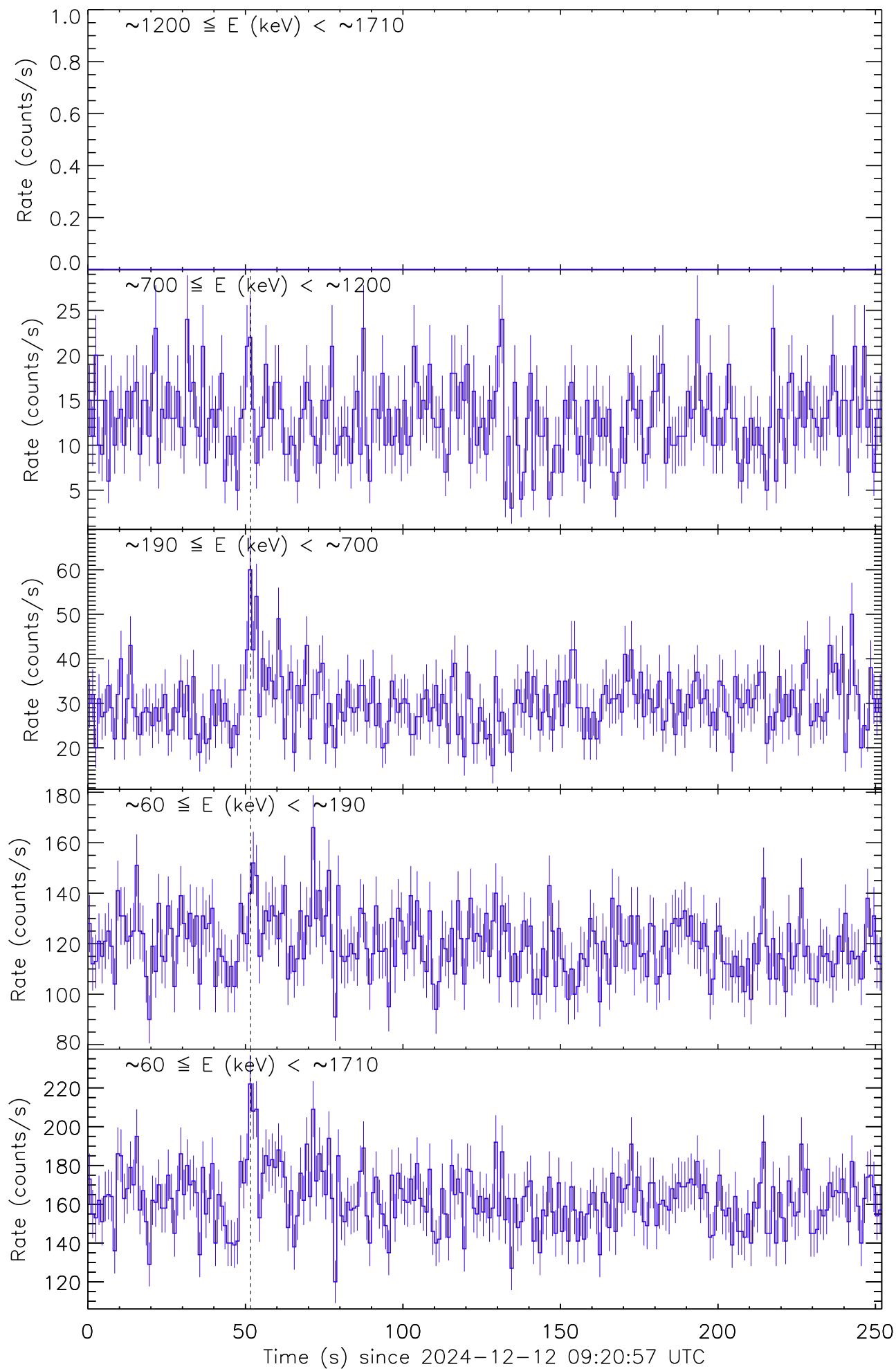
Figure 1: Raw count rate curves of GRB 241212A recorded by the detector unit no. 1. The vertical dashed line marks the trigger time by Fermi/GBM.
