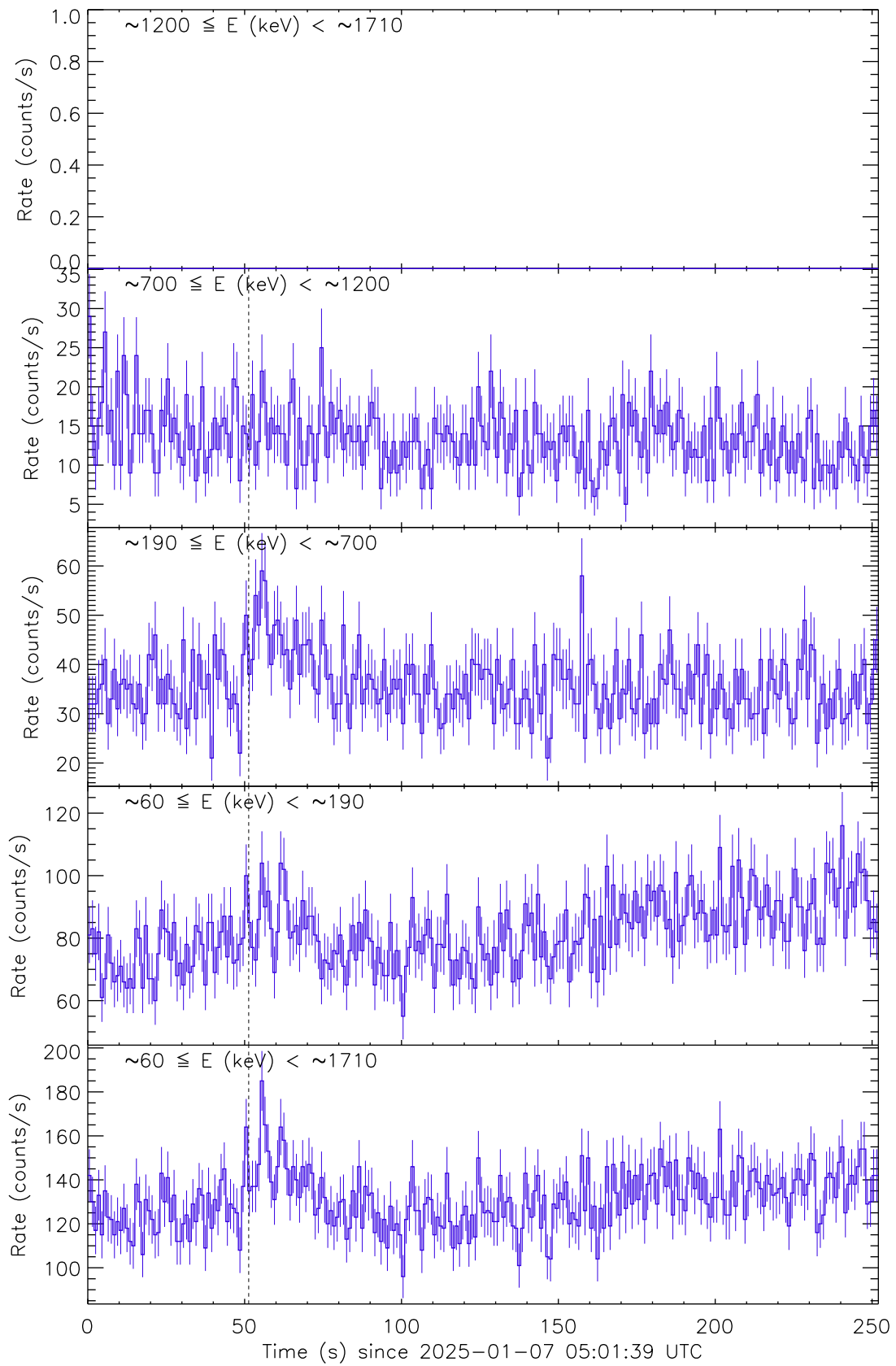
Figure 1: Raw count rate curves of GRB 250107A recorded by the detector unit no. 1. The vertical dashed line marks the trigger time by Fermi/GBM.
