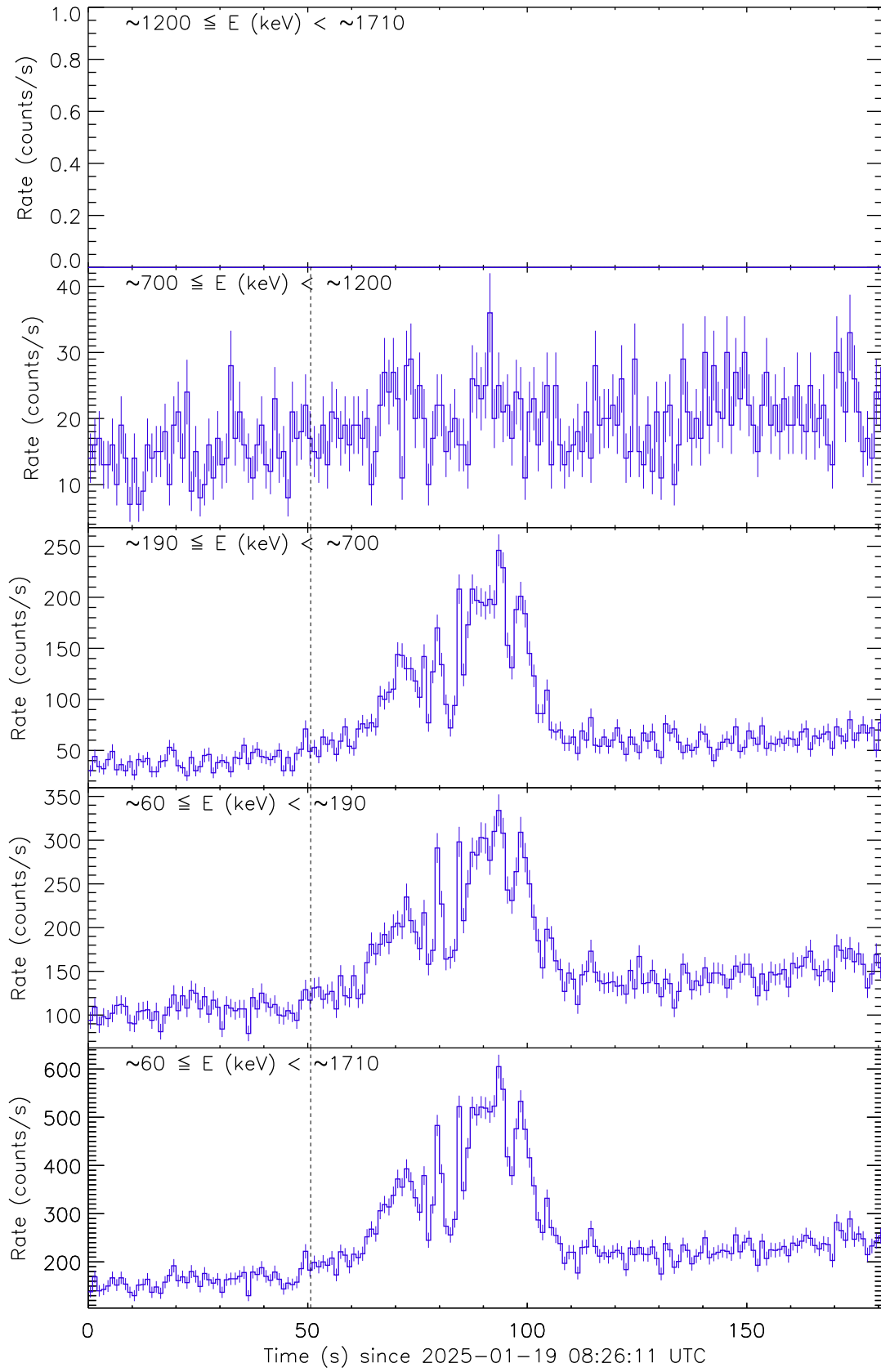
Figure 1: Raw count rate curves of GRB 250119B recorded by the detector unit no. 1. The vertical dashed line marks the trigger time by Fermi/GBM.
