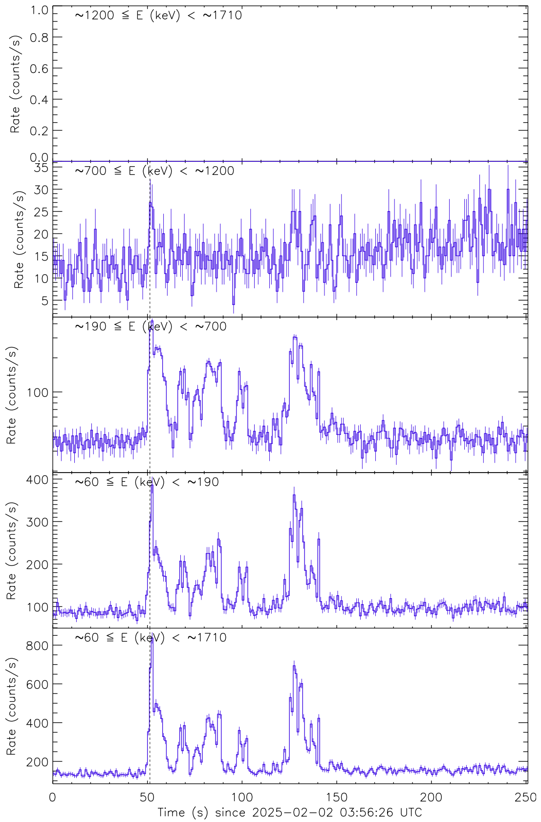
Figure 1: Raw count rate curves of GRB 250202B recorded by the detector unit no. 1. The vertical dashed line marks the trigger time by Fermi/GBM.
