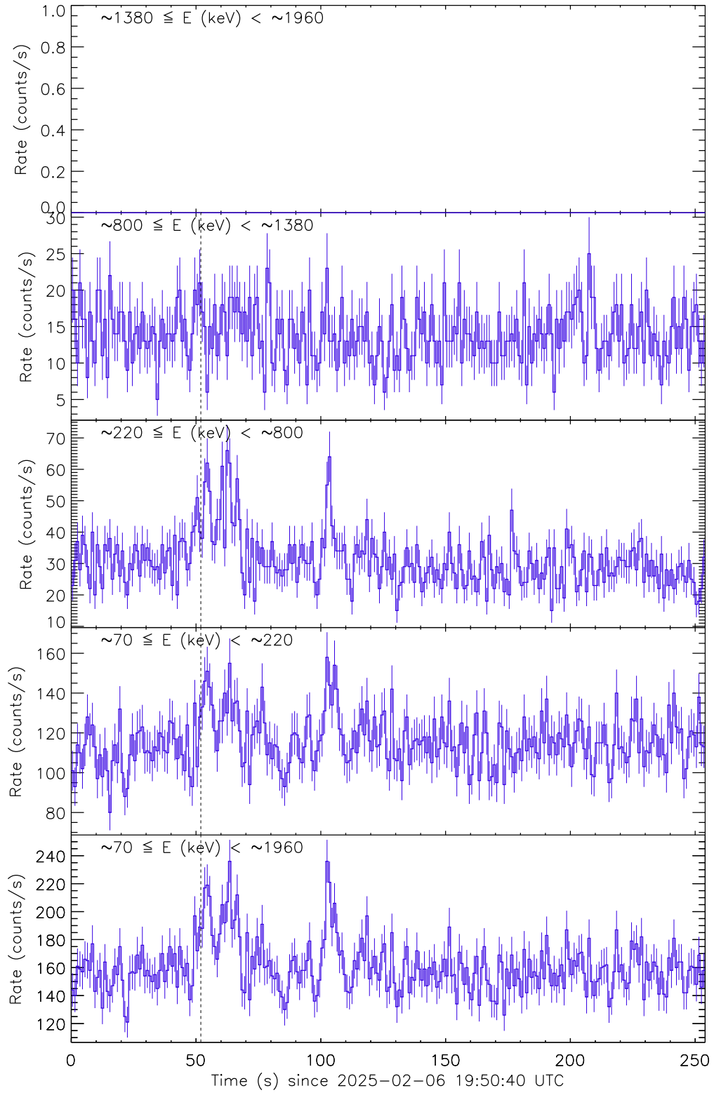
Figure 1: Raw count rate curves of GRB 250206A recorded by the detector unit no. 0. The vertical dashed line marks the trigger time by Fermi/GBM.
