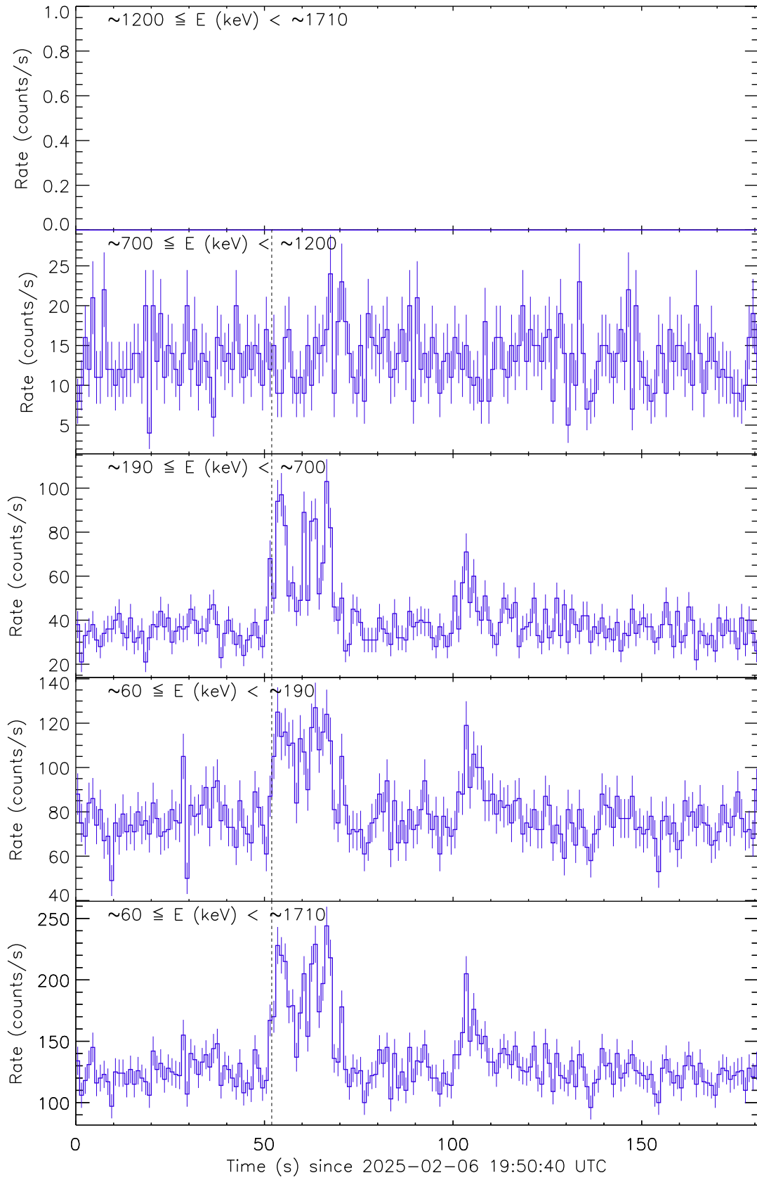
Figure 4: Raw count rate curves of GRB 250206A recorded by the detector unit no. 1. The vertical dashed line marks the trigger time by Fermi/GBM.
