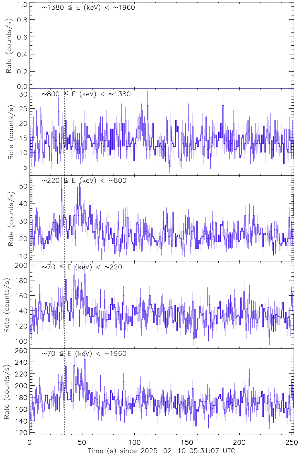
Figure 1: Raw count rate curves of GRB 250210A recorded by the detector unit no. 0. The vertical dashed line marks the trigger time by Fermi/GBM.
